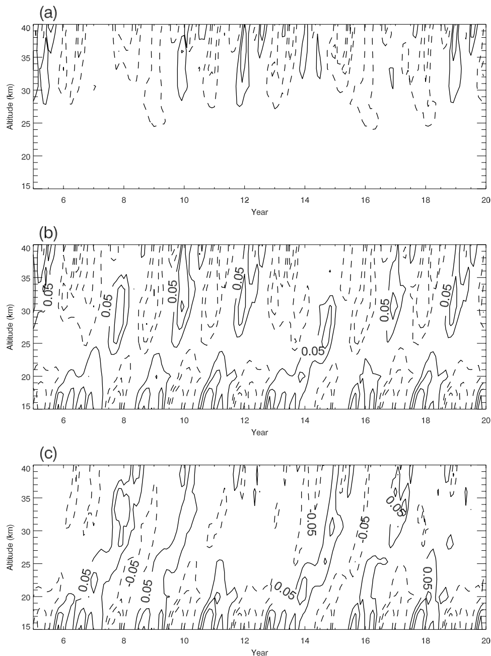
Figure 17. Altitude–time plot of QBO anomalies in equatorial \text{H}_2\text{O} mixing ratio from model simulations (a) W2 and (b) W3 and their difference (c). Contours are drawn every \pm 0.05 , 0.1, 0.2, and 0.3 ppmv, with dashed lines for negative values.
