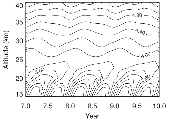
Figure 3. Annual cycle in model stratospheric \text{H}_2\text{O} at the equator from the Q_0 simulation using the fixed lower boundary condition. Contour interval is 0.2 ppmv.
