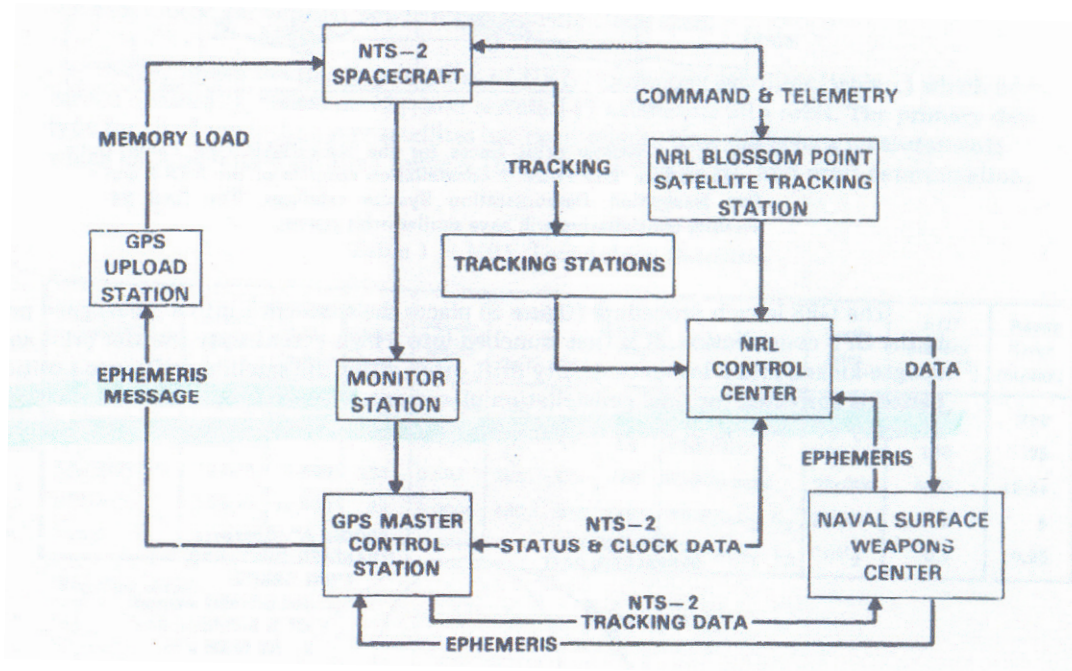
Figure 3-5. NTS-2 Command and Telemetry Links (Ref. 1)
