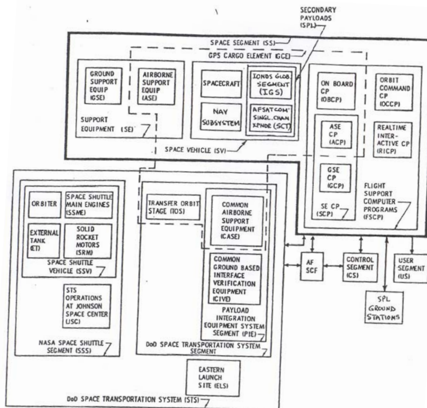
Figure 3-15. Space Segment System Relationship (Ref. 44)
