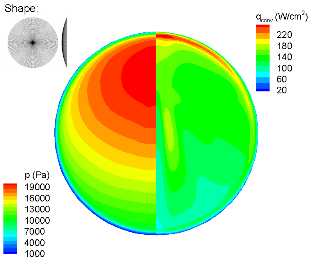
Figure 5.2: Case C (Orion) surface pressure and convective heating profiles
