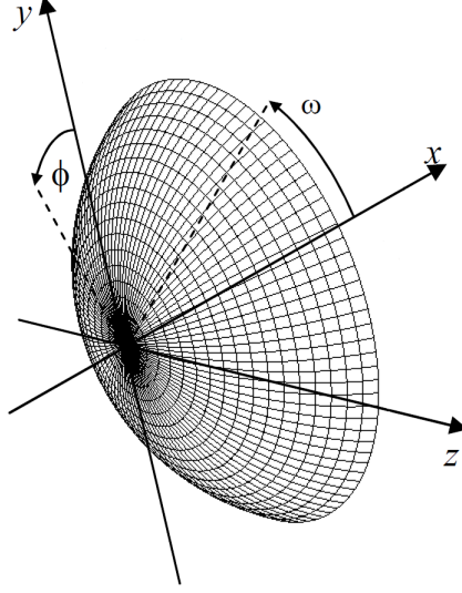
Figure 1.1: Fixed-body coordinate system shown on a 60°axisymmetric spherical segment heat shield
