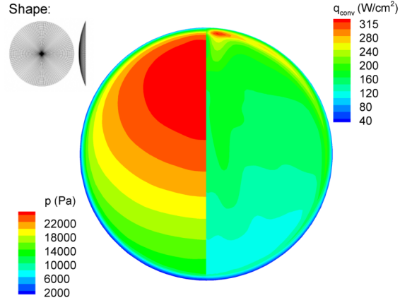
Figure 5.6: Case B (Orion) surface pressure and convective heating profiles
