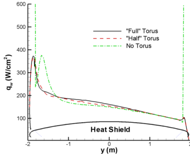
Figure 3.8: Symmetry convective heat flux comparison of Apollo 4 peak heating case for three different torus extents
