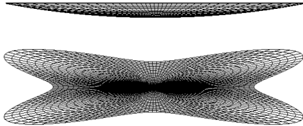
Figure 1.7: Spherical Segment with n_2 = 4.00 , e = .0968 , \theta_s = 15.9^\circ , and \alpha = -12^\circ optimized for minimum q_{s,tot}
