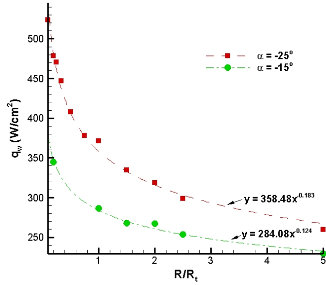
Figure 3.10: Peak convective heat fluxes for Apollo heat shield at Apollo 4 peak heating conditions for two angles of attack
