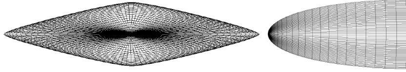
Figure 1.6: Spherical Segment with n_2 = 1.30 , e = -.0968 , \theta_s = 89.0^\circ , and \alpha = 18^\circ optimized for maximum (L_v/D)/q_{s,tot}
