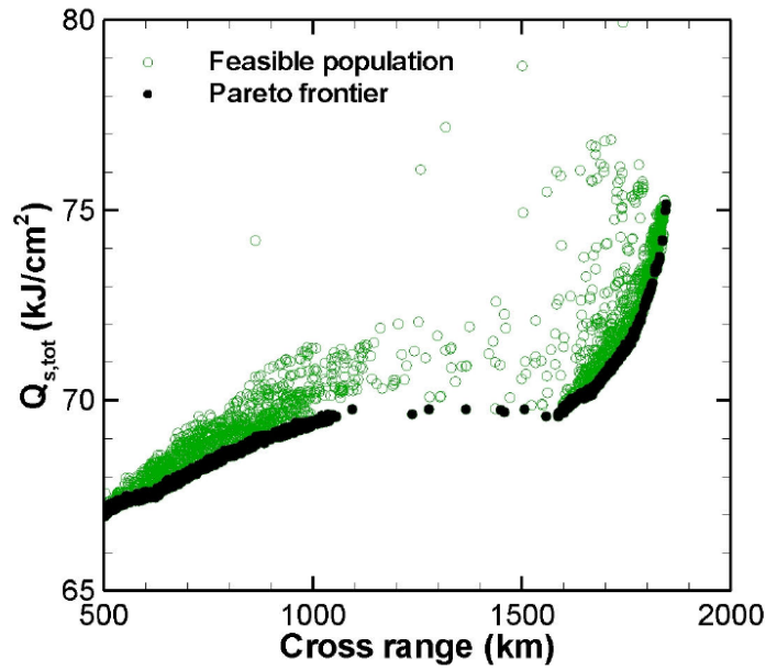
Figure 1.8: Pareto frontier example for a spherical segment ( L/D = 0.5 , V_E = 12.5 km/s)
