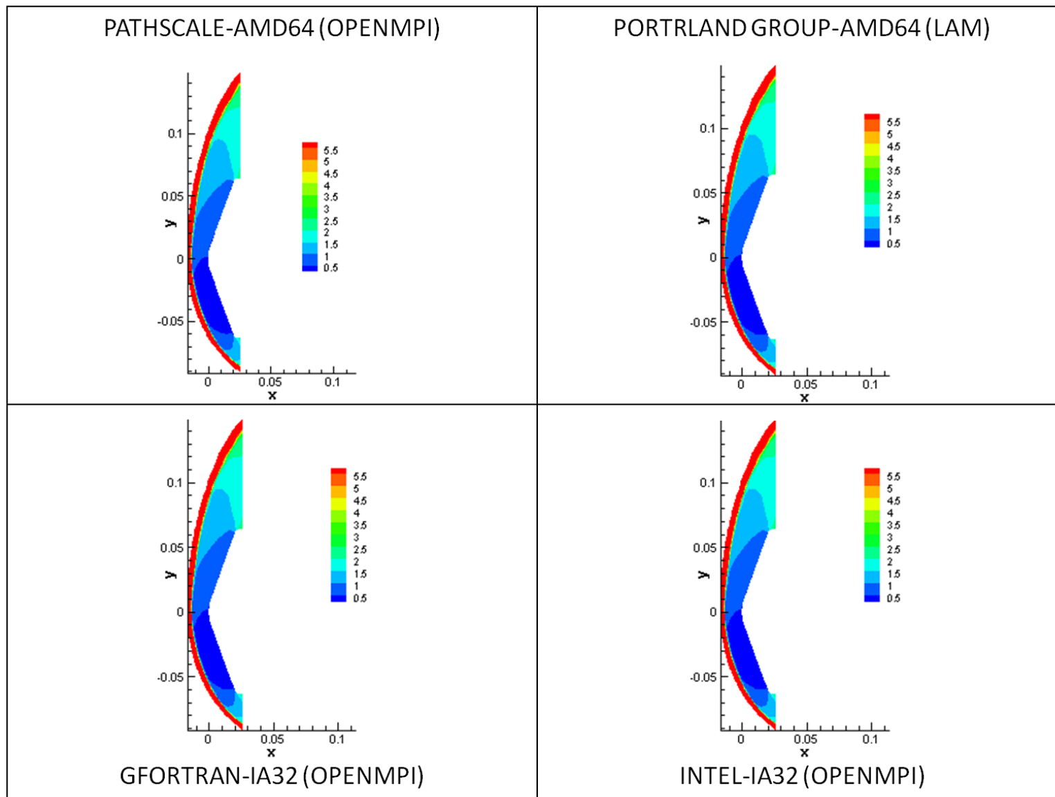
Figure 2.2: Mach number contours on symmetry plane for MSL
