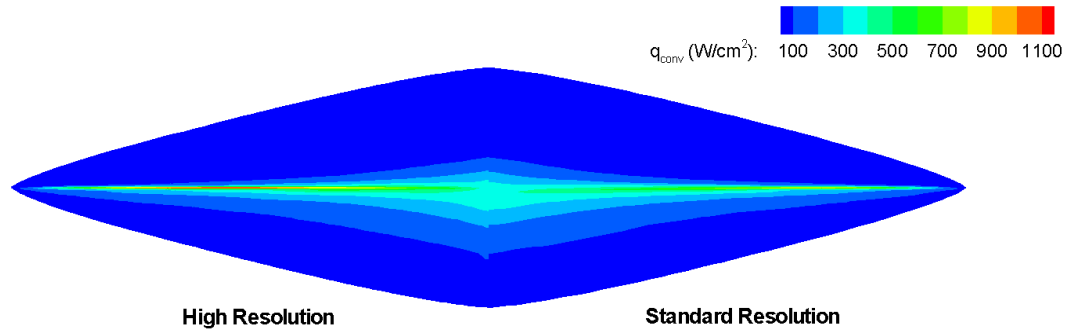
Figure 4.5: Surface convective heat flux for slender heat shield surface grid resolution study
