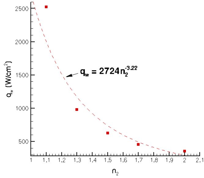
Figure 4.7: Maximum convective heat fluxes for 89° spherical segment with varying n_2 parameter
