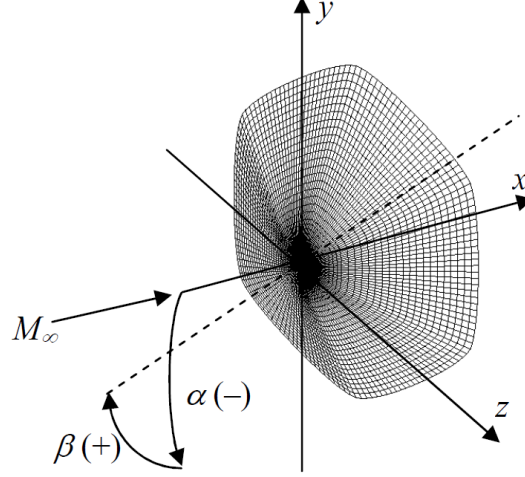
Figure 1.5: Freestream coordinate system for \alpha and \beta
