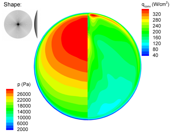
Figure 5.7: Case F (Orion) surface pressure and convective heating profiles
