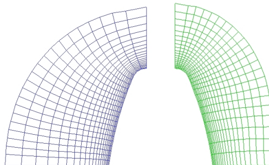
Figure 2.5: Edge spacing for the Apollo heat-shield
