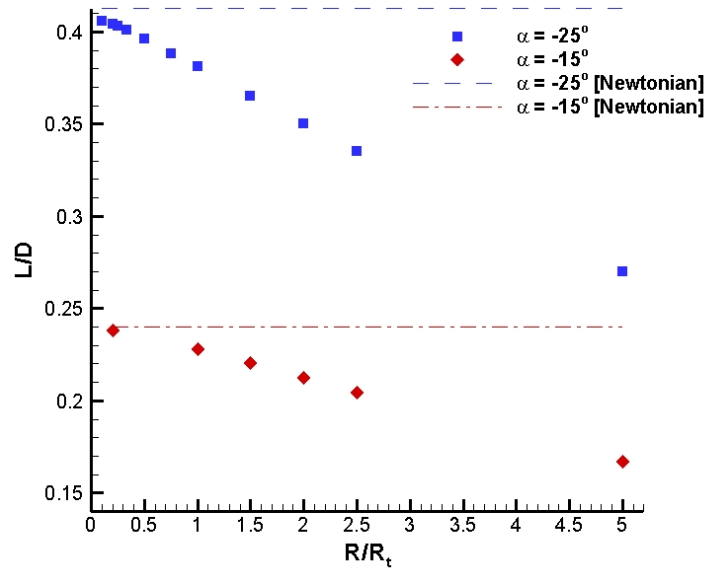
Figure 3.11: Lift to drag ratios versus torus radius for Apollo heat shield at two angles of attack
