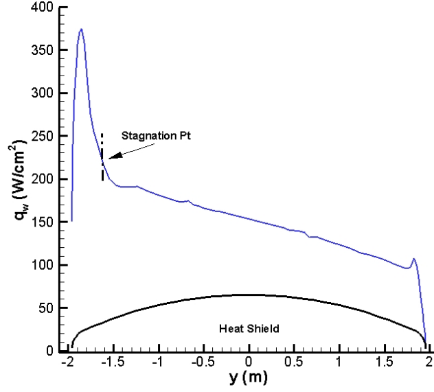
Figure 3.4: Symmetry line heating profile for Apollo 4 at peak heating conditions
