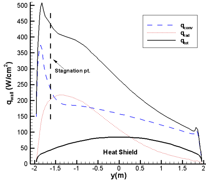
Figure 3.7: Convective, radiative, and total heat flux on symmetry plane for Apollo heat shield at Apollo 4 peak heating conditions
