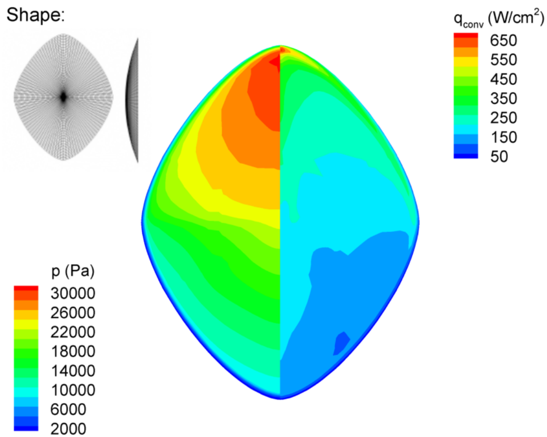
Figure 5.5: Case A surface pressure and convective heating profiles
