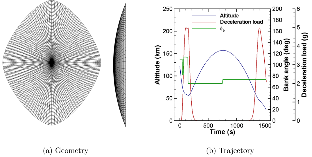
Figure 1.10: Spherical segment with \theta_s = 23.7^\circ , n_2 = 1.66 , and e = 0.621 optimized for Lunar Return ( V_E = 12.5 \text{ km/s} )
