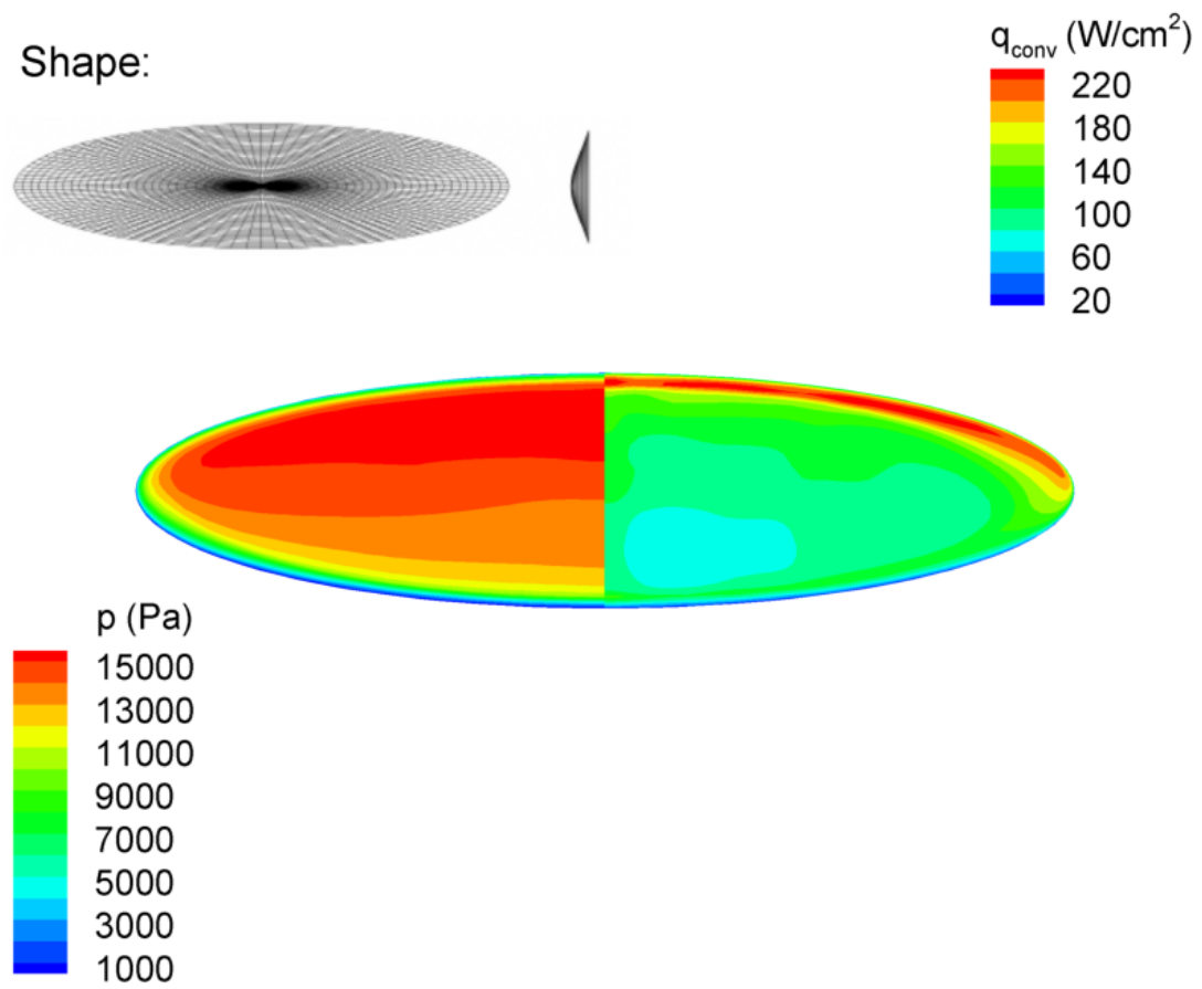
Figure 5.8: Case D surface pressure and convective heating profiles
