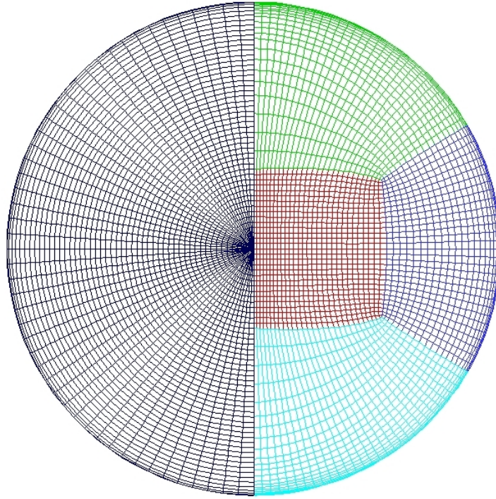
Figure 2.4: Nose patching as shown on the Apollo heat-shield
