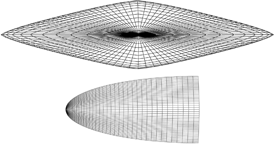
Figure 4.1: 89° spherical segment with n_2 = 1.3 optimized for maximum L/D
