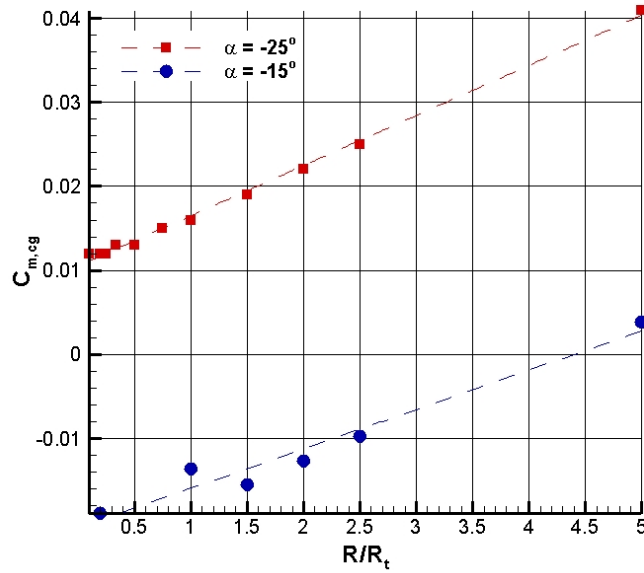
Figure 3.12: Moment coefficient for Apollo heat shield at different angles of attack
