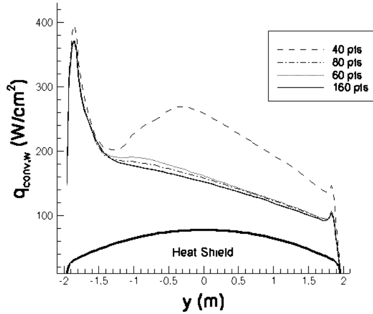
Figure 3.5: Symmetry plane convective heat flux for Apollo heat shield grid resolution study
