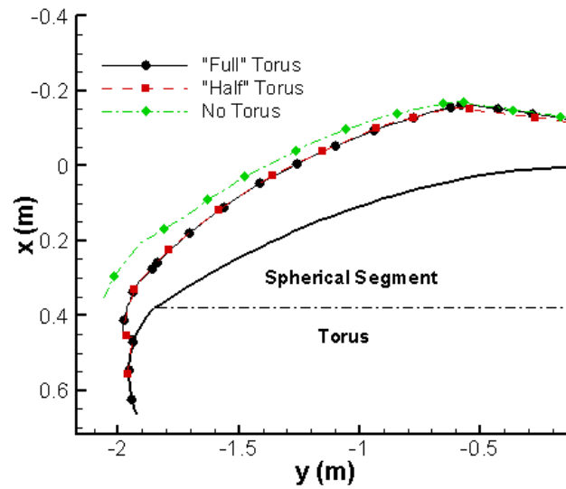
Figure 3.9: Sonic line comparison of Apollo 4 peak heating case for three different torus extents
