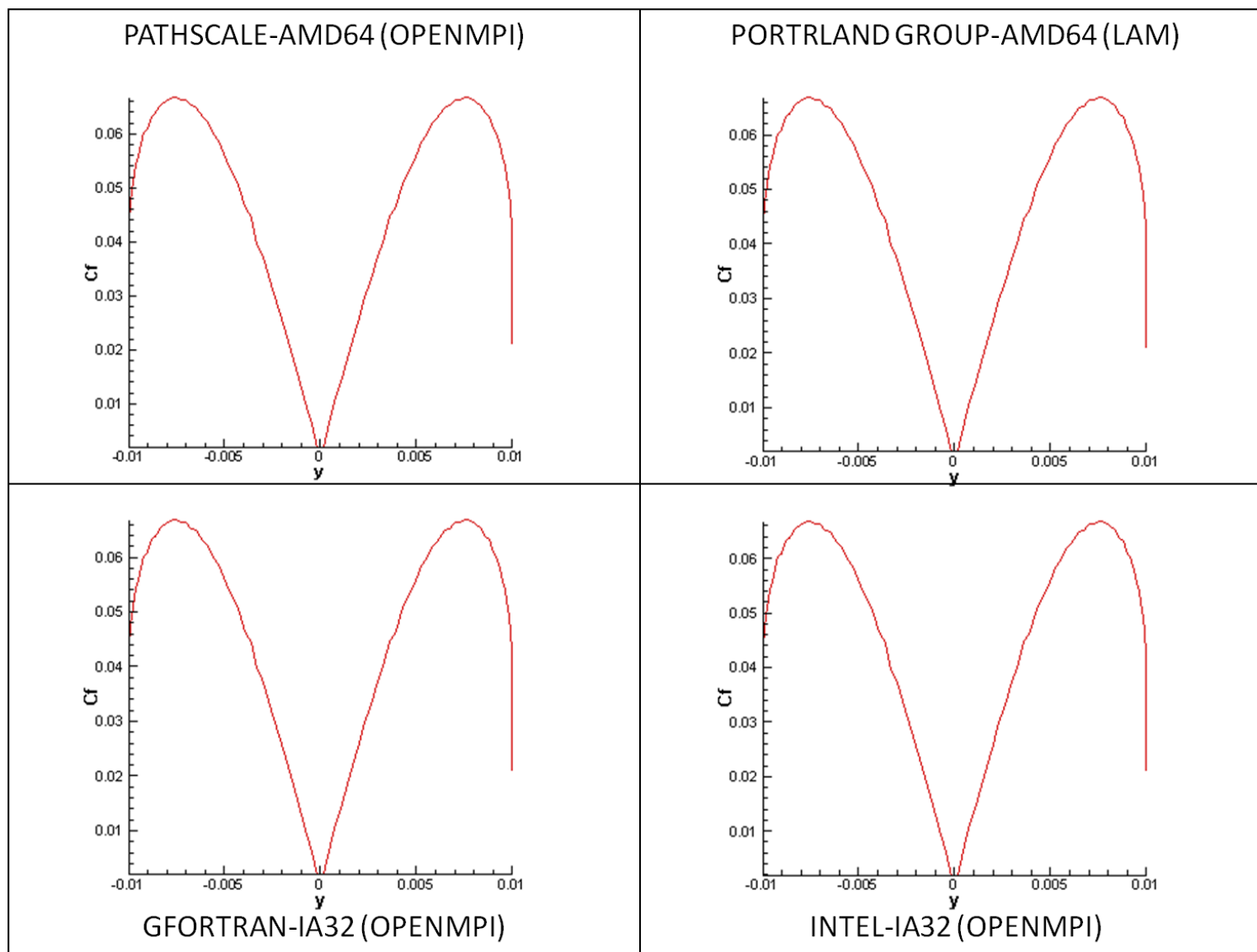
Figure 2.3: Surface skin friction coefficients on a 2-D cylinder
