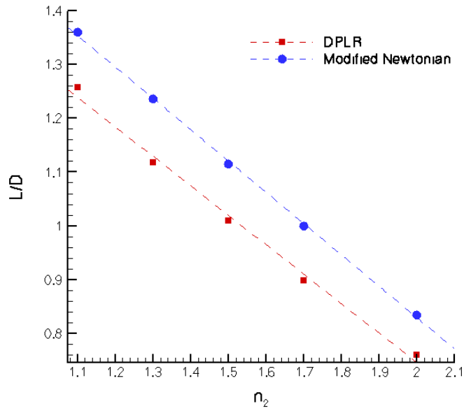
Figure 4.8: Lift to drag ratios for 89° spherical segment with varying n_2 parameter
