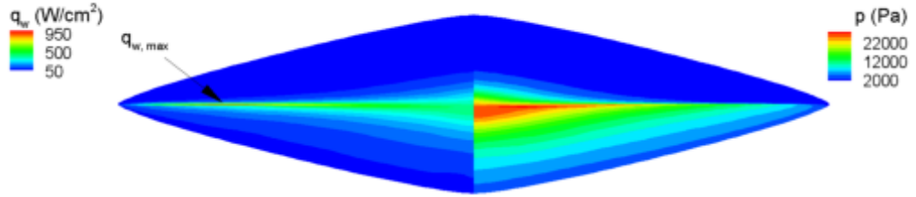
Figure 4.3: Surface convective heat flux and pressure contours for 89° spherical segment optimized for maximum L/D
