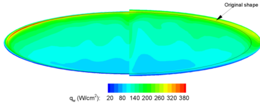
Figure 3.13: Convective heat flux on an elliptical heat shield for two different methods of torus generation
