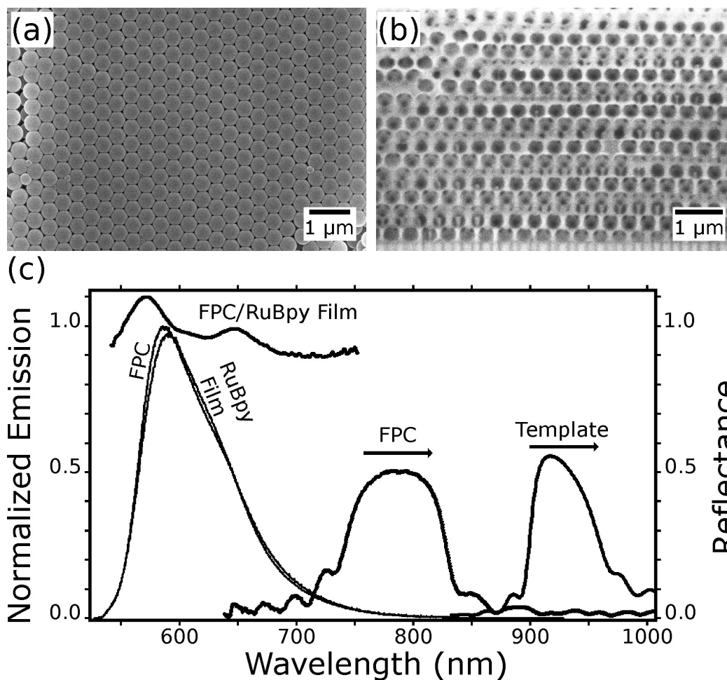
Figure 5. SEM micrographs of (a) polystyrene colloidal template and (b) FPC cross-section. (c) Normalized emission spectra, integrated over 76% of 2\pi sr, from FPC, RuBpy film, and their ratio. Also in (c), normal-incidence reflectance from FPC and template.
