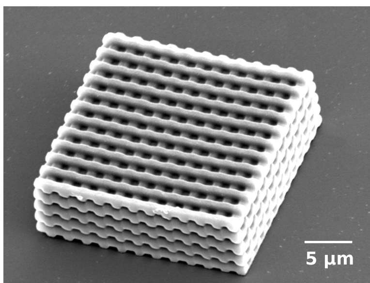
Figure 1. Scanning electron micrograph of the highest quality woodpile structure fabricated in SU8 photo-resist using direct laser writing.
