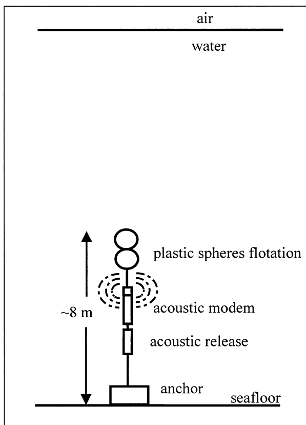
FIG. 3. Near-bottom in-line mooring configuration for network nodes consisting of individual acoustic modems only (referred to as repeaters and listeners).
