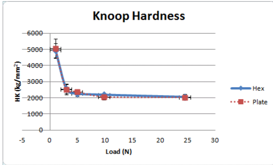
Figure 5. Load-HK curve.
