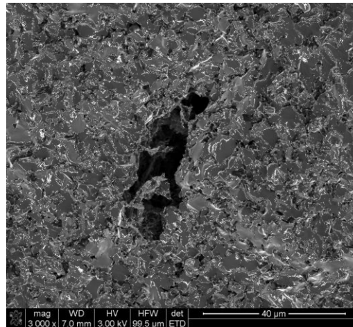
Figure 4. SEM of pore in the weakest sample.
