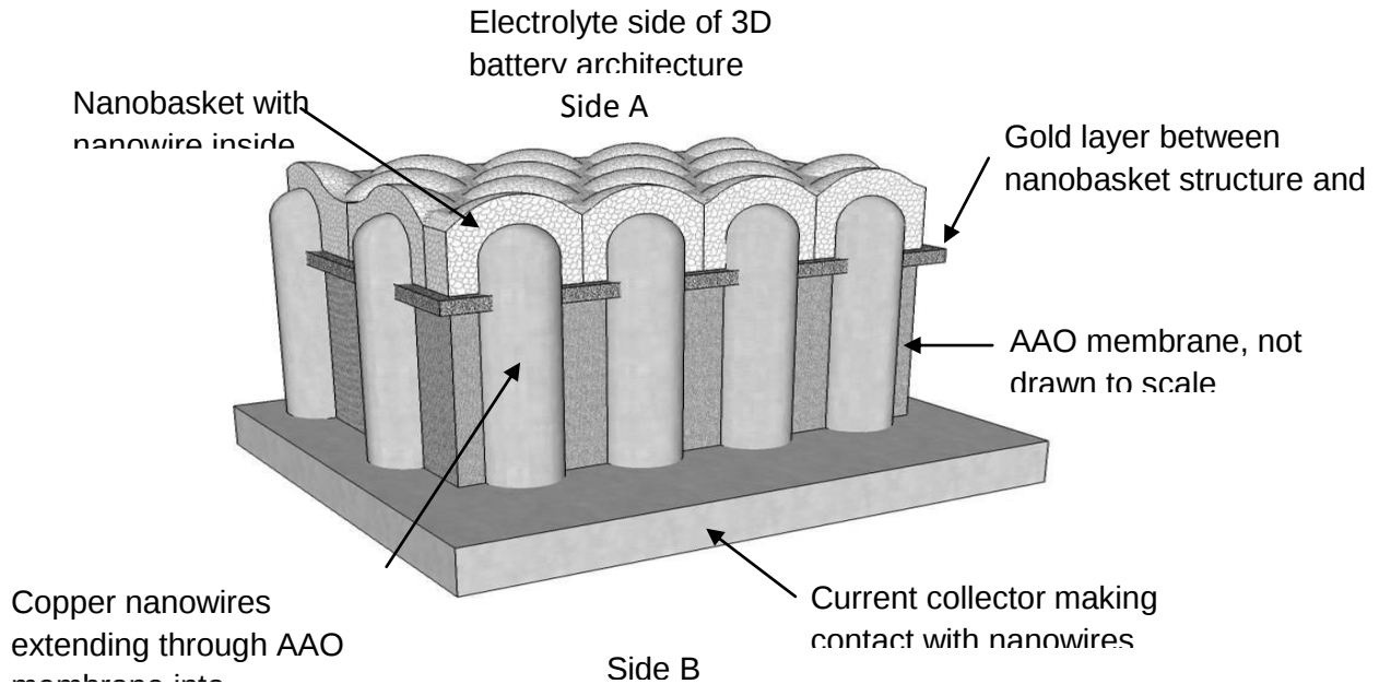
Fig. 12. Schematic of 3D nanobattery architecture.
