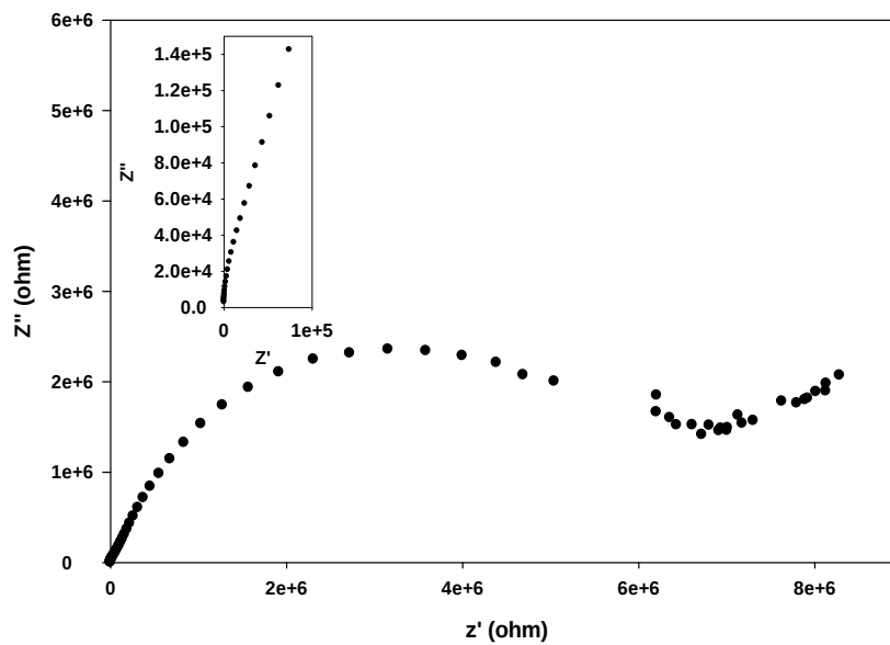
Fig. 15. Nyquist plot of the nanobasket layer. The inset shows the high frequency region in more detail.
