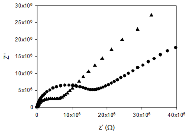
Fig. 22. Nyquist plots for PEO confined in a nanoporous AAO membrane ( \blacktriangle ) and non-confined PEO ( \bullet )
