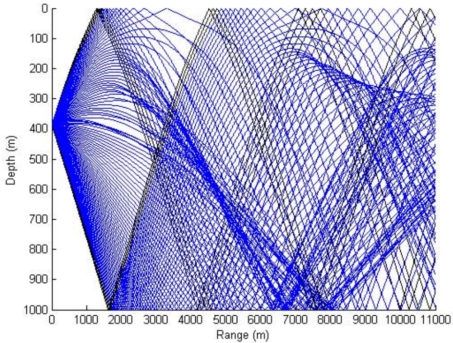
Figure 34. Ray trace for a source at 387 m in a smoothed profile.
