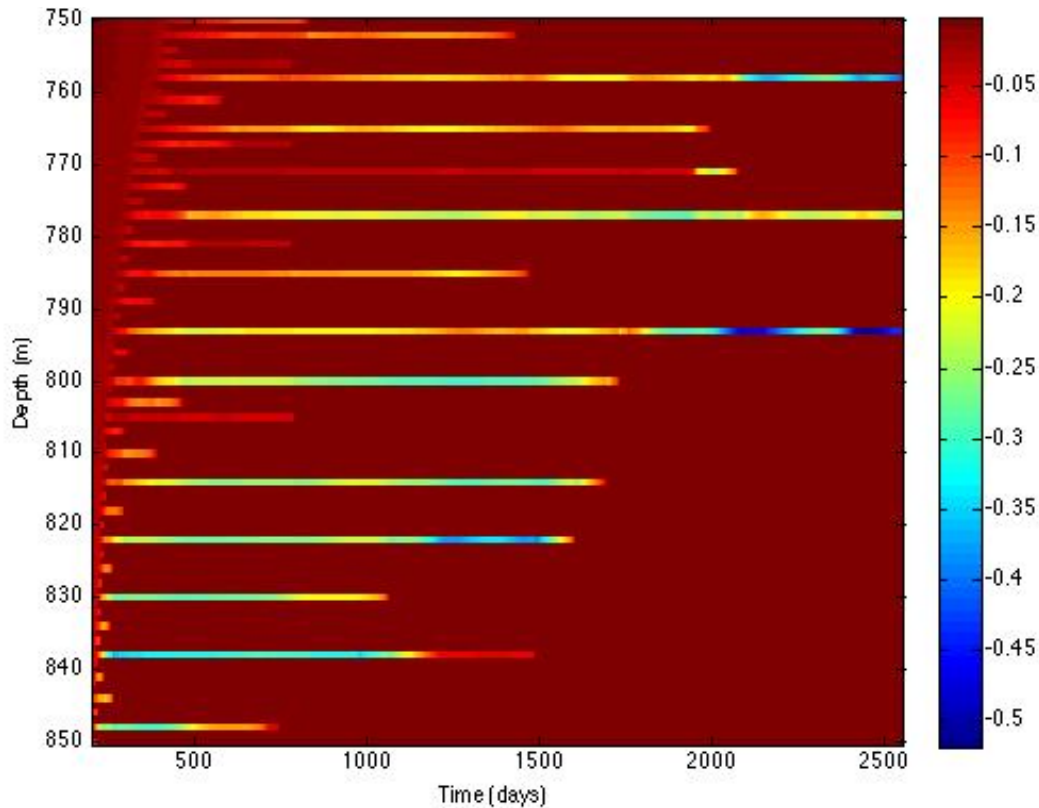
Figure 20. Space-time diagram of the numerically modeled temperature gradient ( ^{\circ}C/m ). Layers merge when the relatively strong interfaces grow further at the expense of weaker interfaces, which decay and eventually disappear (B-merger scenario).
