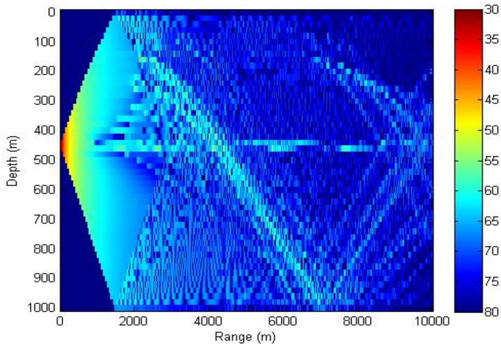
Figure 45. Coherent TL (dB/m) for stepped profile with 2000 Hz source in layer.
