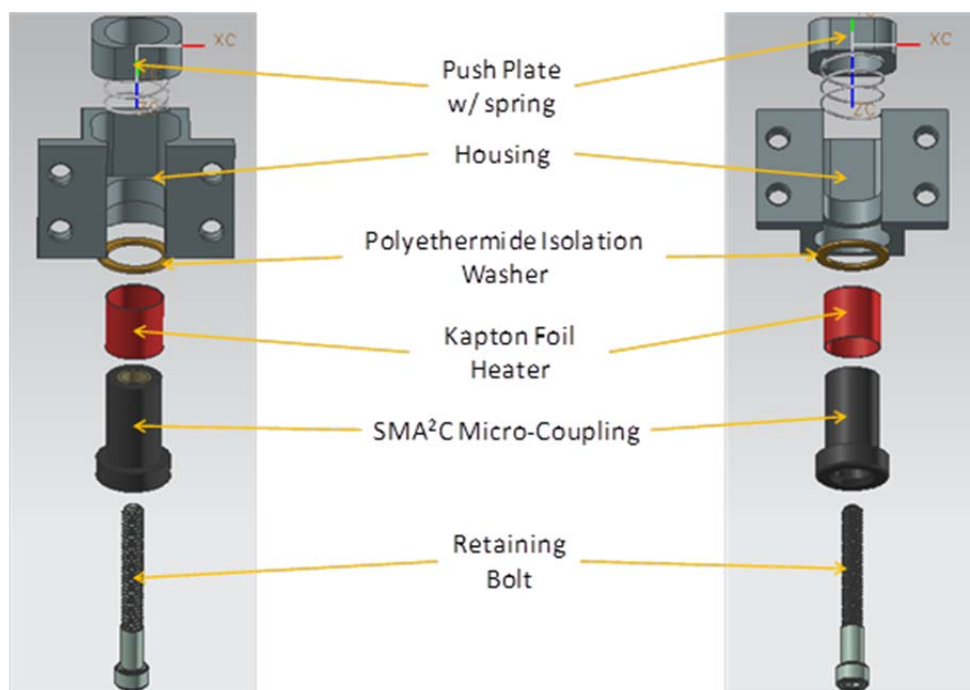
Figure 15. Component View of SMA 2 C Device. From [4]
