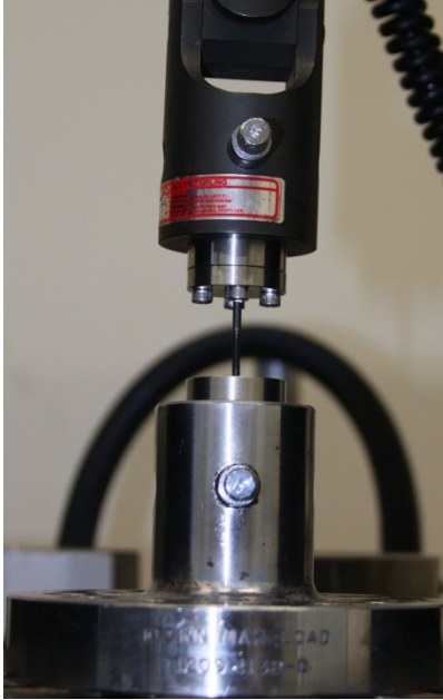
Figure 40. Separation Testing
