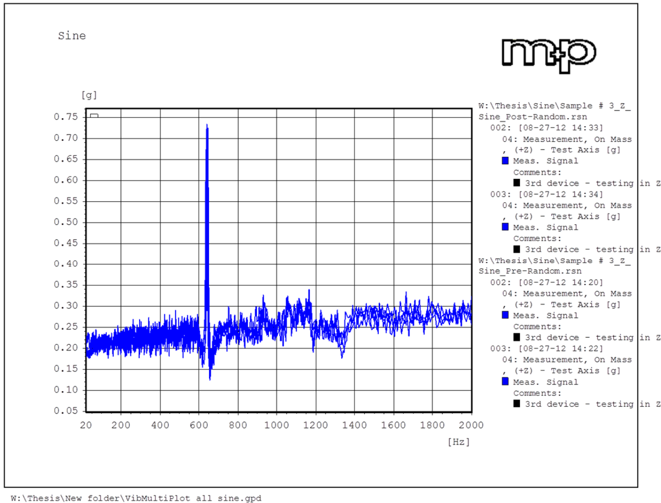
Sample 3 Pre and Post sine plot in the Z-Axis
