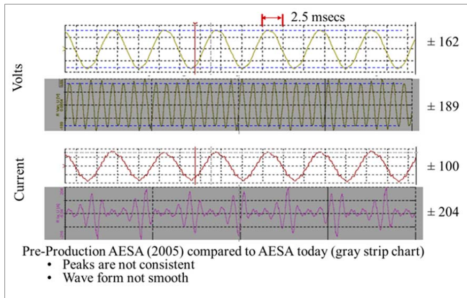
Figure 1. Generator Converter Unit's Current Utilization (From Commander, 2010)
