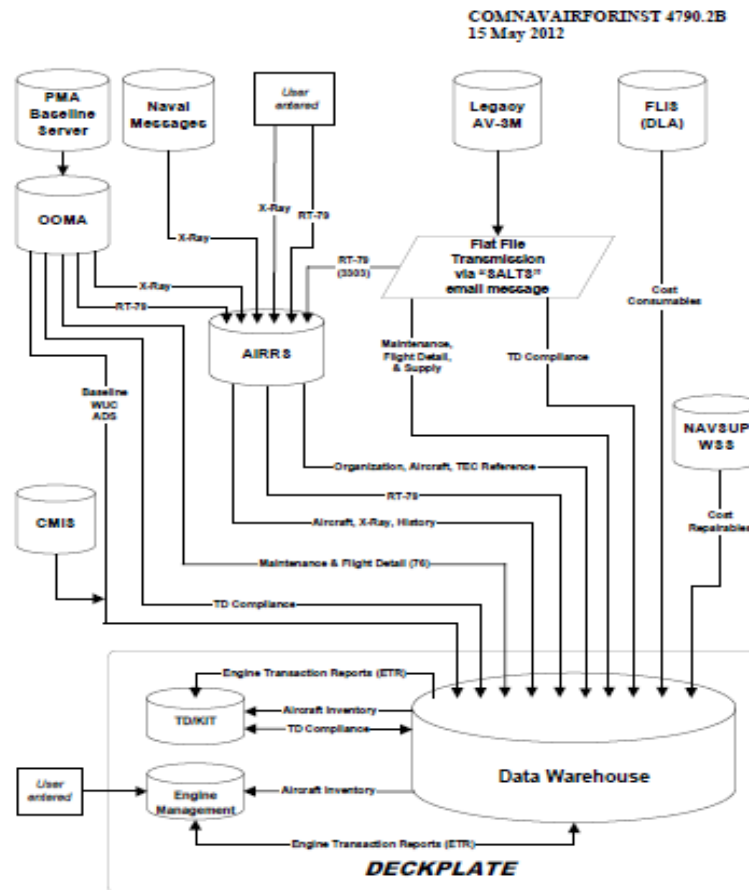
Figure 2. DECKPLATE Data Flow (From COMNAVAIRFORINST, 2012).
