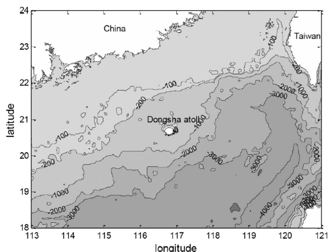
Fig. 1. Location of the Dongsha atoll and bathymetry (unit: m) in the northeastern SCS.
