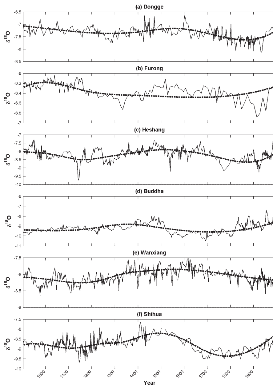
Figure 3. Time series of high-resolution (yearly) speleothem \delta^{18}\text{O} data from south to north at the (a) Dongge, (b) Furong, (c) Heshang, (d) Buddha, (e) Wanxiang and (f) Shihua caves. Here, the dashed curves represent the trends obtained using the EMD method. It is noted that all the trends show a similar pattern (except the recent increase of speleothem \delta^{18}\text{O} since 1800 except at the Wanxiang cave).
