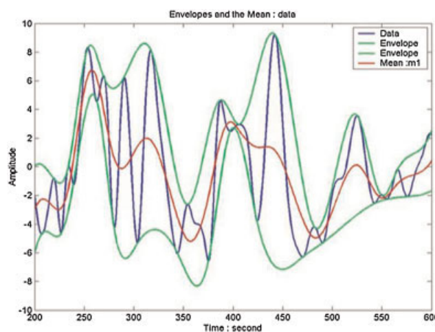
Figure 4. Illustration of the EMD process, with the blue curve denoting x(t) , the two green curves representing envelopes of local maxima e_{\max}(t) and minima e_{\min}(t) and the red curve referring to m_1(t) = [e_{\max}(t) + e_{\min}(t)]/2 .
