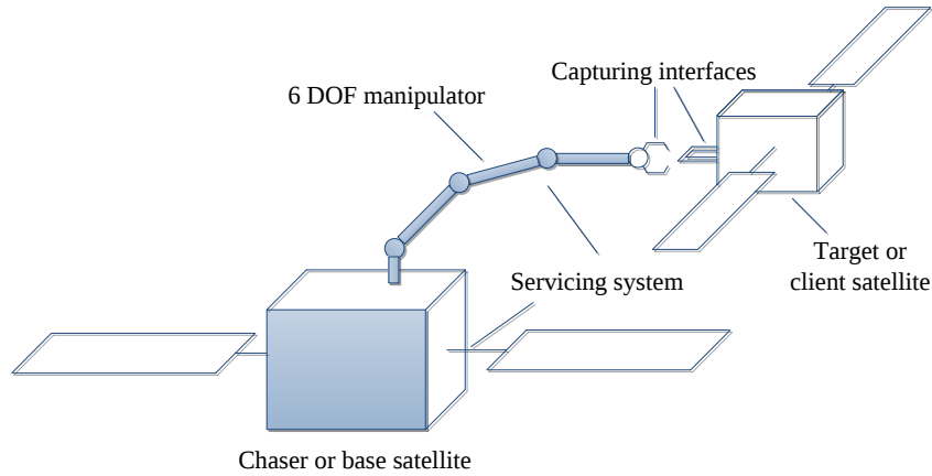
Figure 3. Components of a Space Manipulator for On-orbit Servicing.
