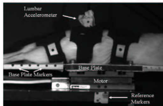
Fig. 1. Experimental set up imaged using CCD camera showing base plate, motor, lumbar accelerometer, and markers.
