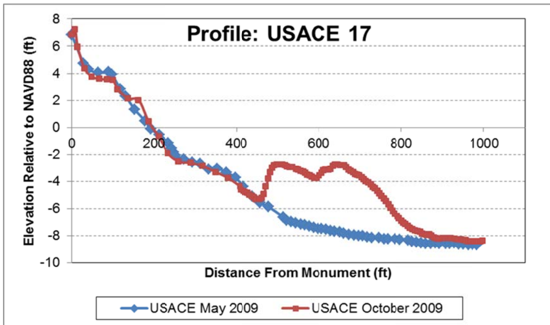
Figure 39. Profile at USACE 17. Note the small gap created during construction.
