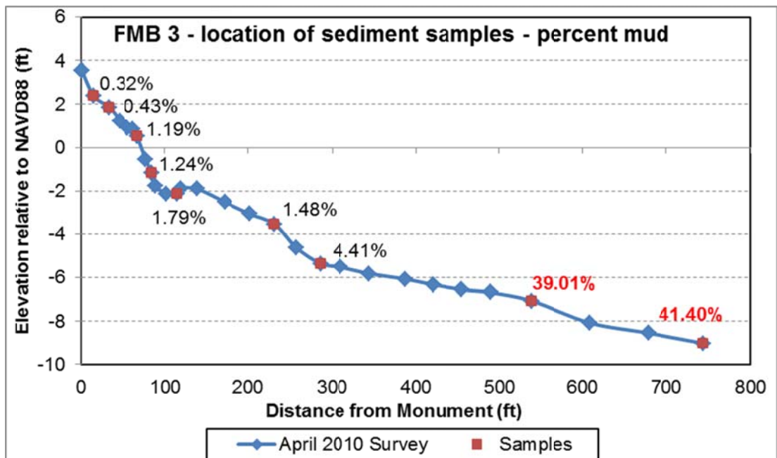
Figure 14. Beach Profile of FMB 3 with Sediment Sample Locations and Mud Percentages.
