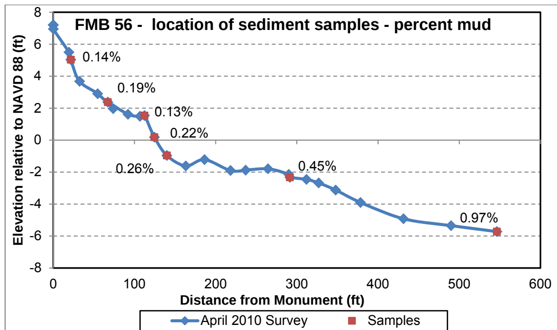
Figure D12. Sample Locations with Mud Percentages at FMB 56.
