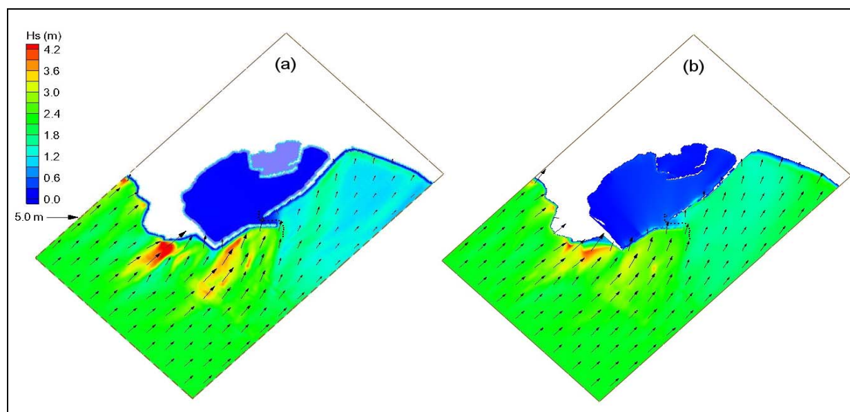
Figure 4. Calculated wave fields by (a) BOUSS-2D, and (b) CMS-Wave at Pillar Point Harbor for H_s = 2 m, T_p = 14 sec, \theta_p = 225 deg (from SE)
