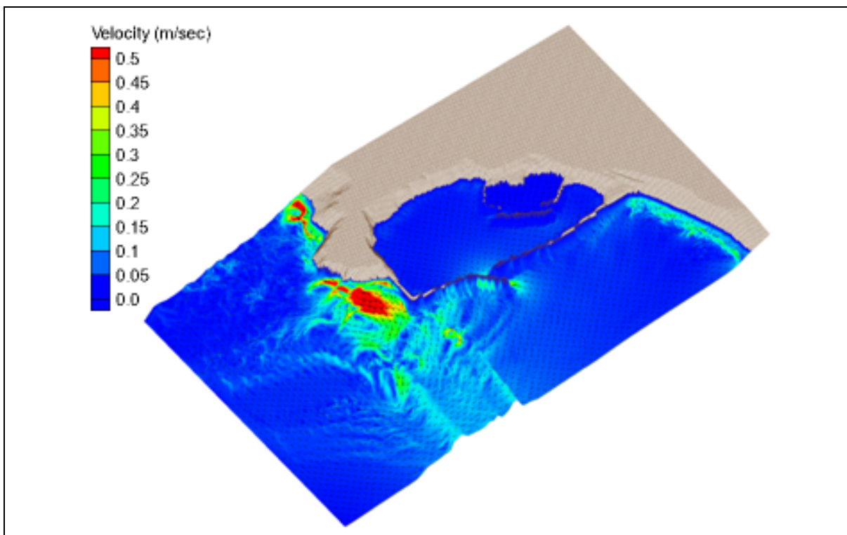
Figure 6. BOUSS-2D calculated wave-induced current vector field.
