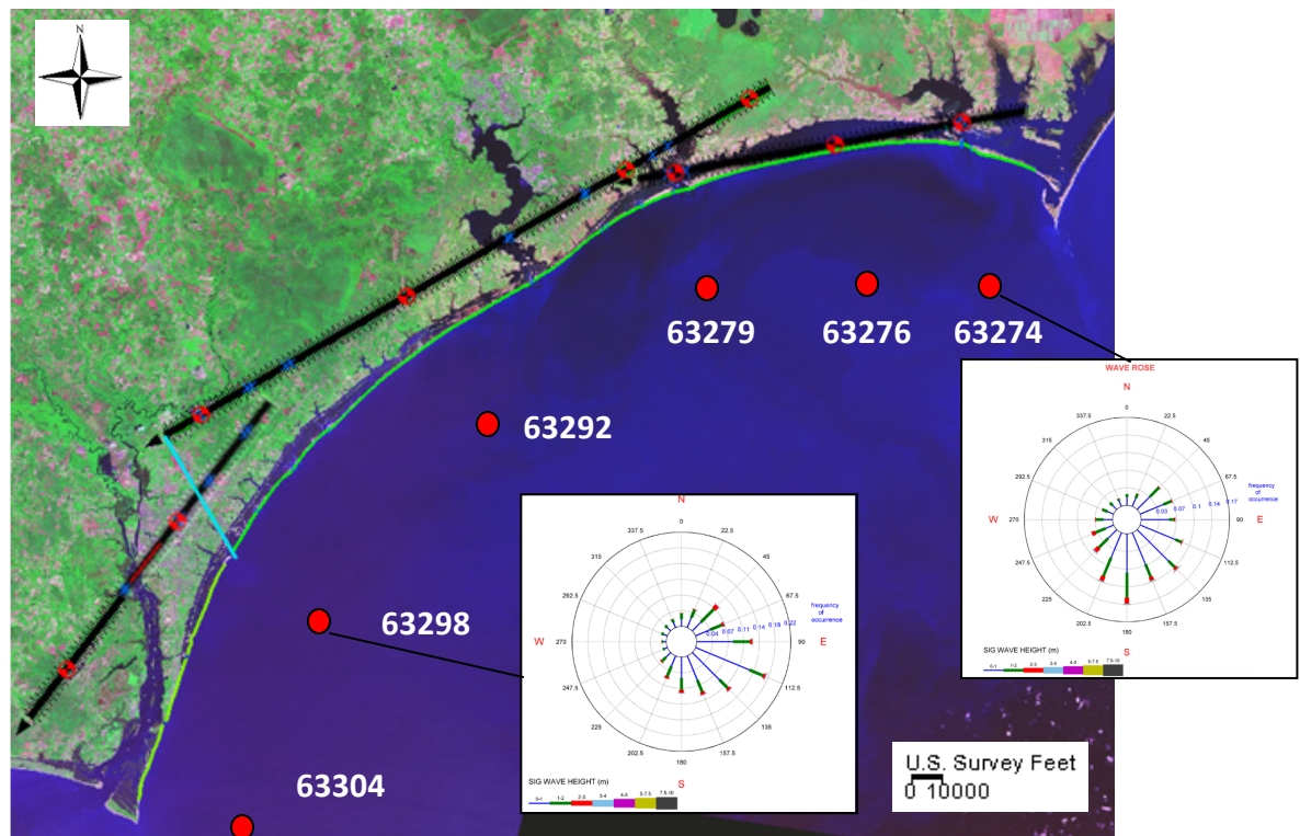
Figure 2. Primary Grid in Center, Secondary Grids in upper right and lower left. WIS wave stations used as input (red circles) and wave roses for stations 63274 and 63298 are also presented.
