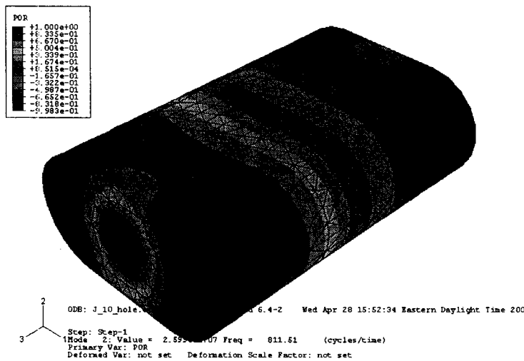
Figure 9. First acoustic cavity mode (no pipe ends).
