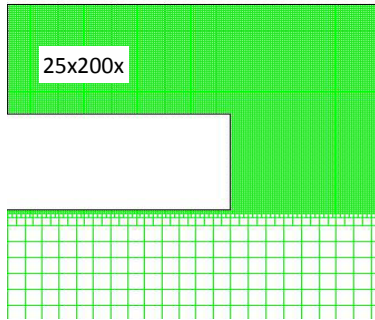
Figure 5b. Mixed Meshing - Localized Refinement Figure 5. Mesh Progression (2D), 25x~250 \mu\text{m} ; 200x ~ 30 \mu\text{m}
