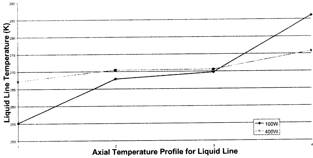
Figure 5: Data showing different liquid line temperature profiles as a function of power at -20°C Sink.
