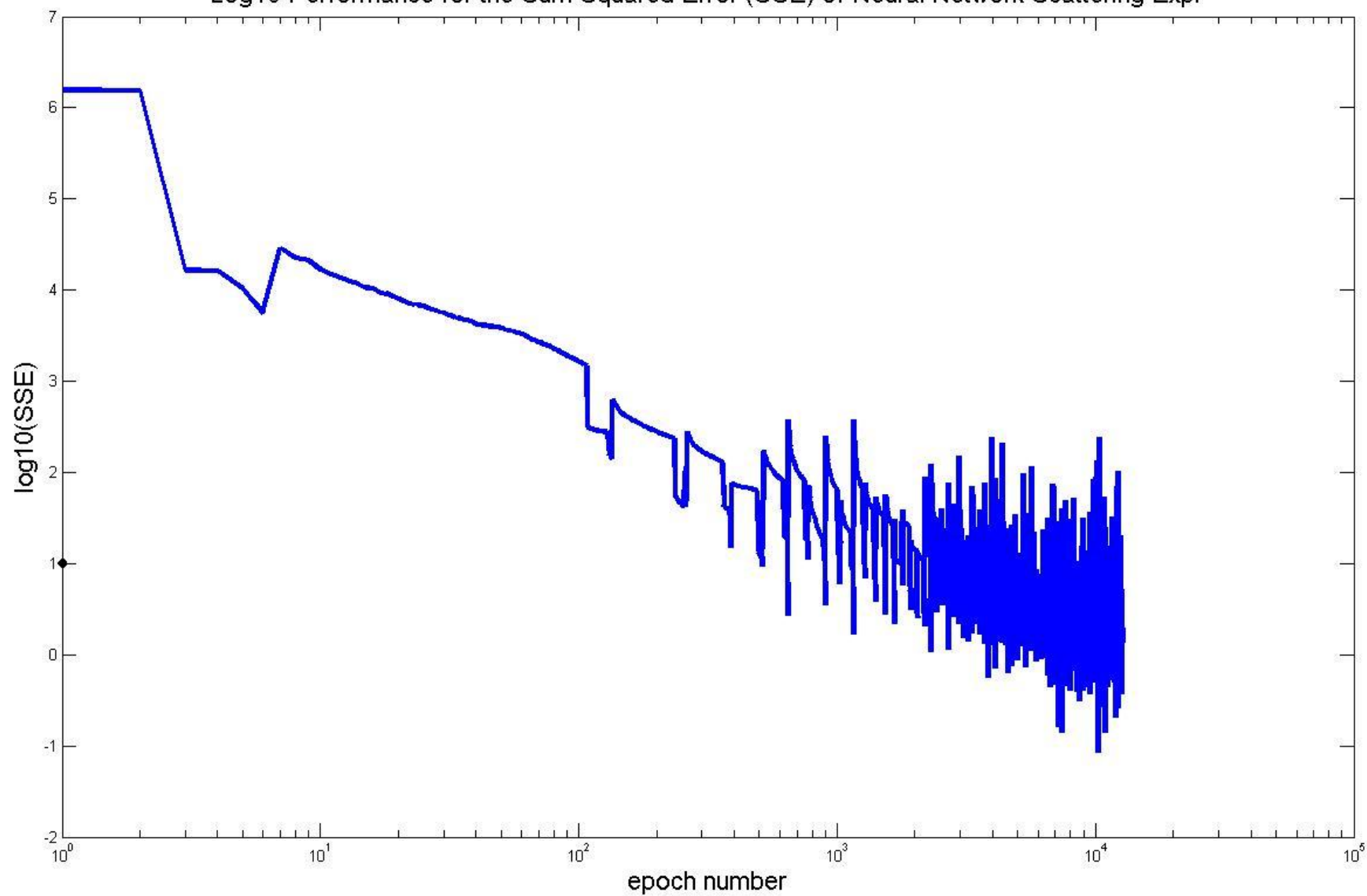
Log10 Performance for the Sum Squared Error (SSE) of Neural Network Scattering Expr
