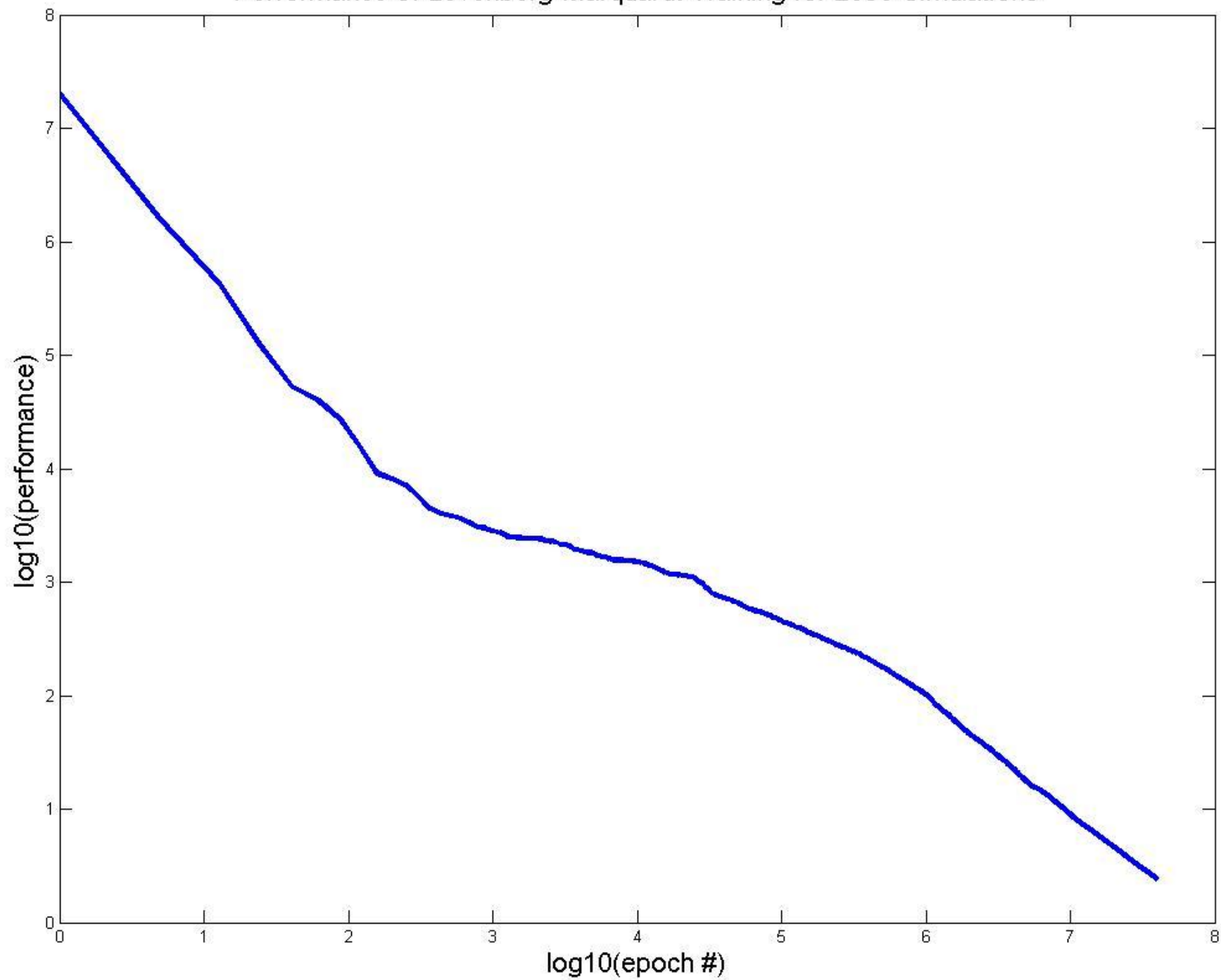
Performance of Levenberg-Marquardt Training for 2856 Simulations
