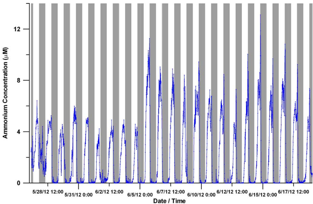
Figure 6. Measurement of ammonium concentration in the surface waters of the pond under the AOML/NOAA building from May 26 to June 19, 2012.
