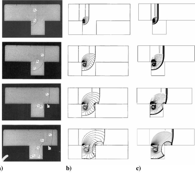
Figure 7. Shock Wave Interacting with a Square Cavity at M_S = 2.032 . Experimental schlieren/shadowgraphs taken from Igra et al. 1996 88 . b) Numerical isopycnics taken from Igra et al. 1996 88 c) Numerical isopycnics produced from current numerical methods.
