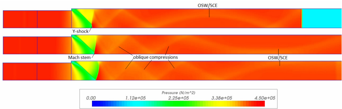
Figure 17. Full-Solution Pressure Map for Case (1.93, 1.1)
