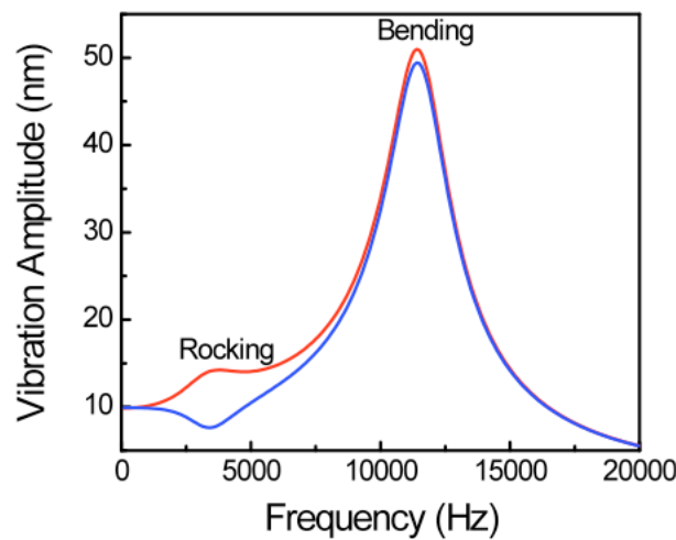
Figure 4. Theoretical frequency response of the fly's hearing organ (From [1]).
