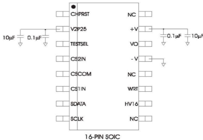
Figure 25. MS3110 IC is presented here with external capacitors.
