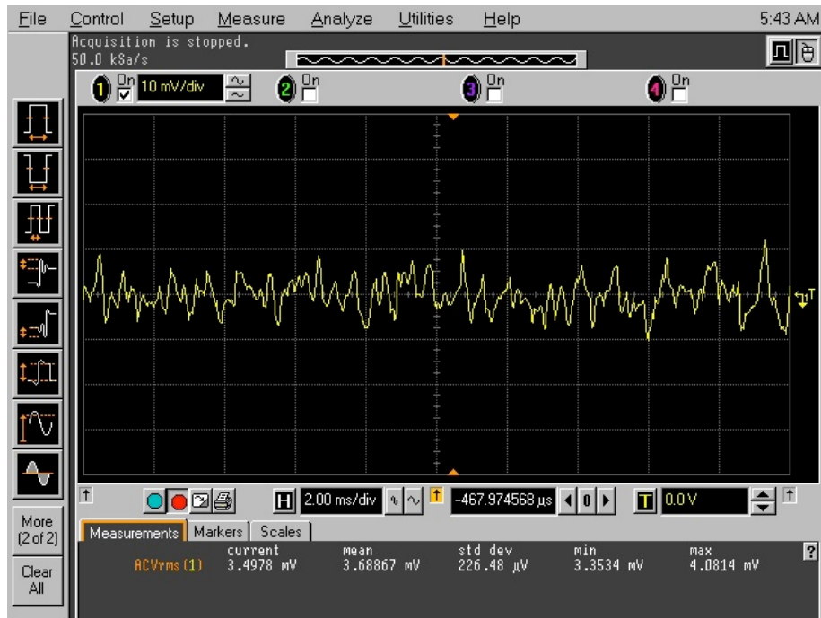
Figure 36. The noise floor with short leads showed a variance lower than the noise floor with long leads.
