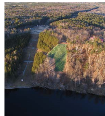
Figure 36. Aerial of finished slope.
