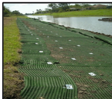
Figure 29. ARVS system installed with anchors.
