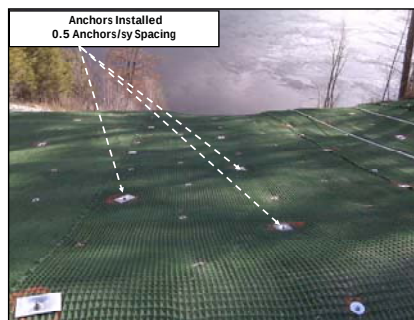
Figure 35. Anchor layout.
