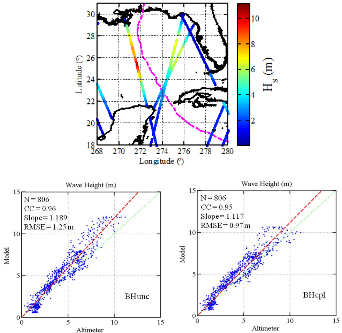
Figure 3.1-10: Satellite altimeter paths with SWH ( H_s ) for 1200 UTC 14 September 2004 forecast (top). Statistical analysis for all N=806 observations for BHunc (bottom left) and BHcpl (bottom right).
