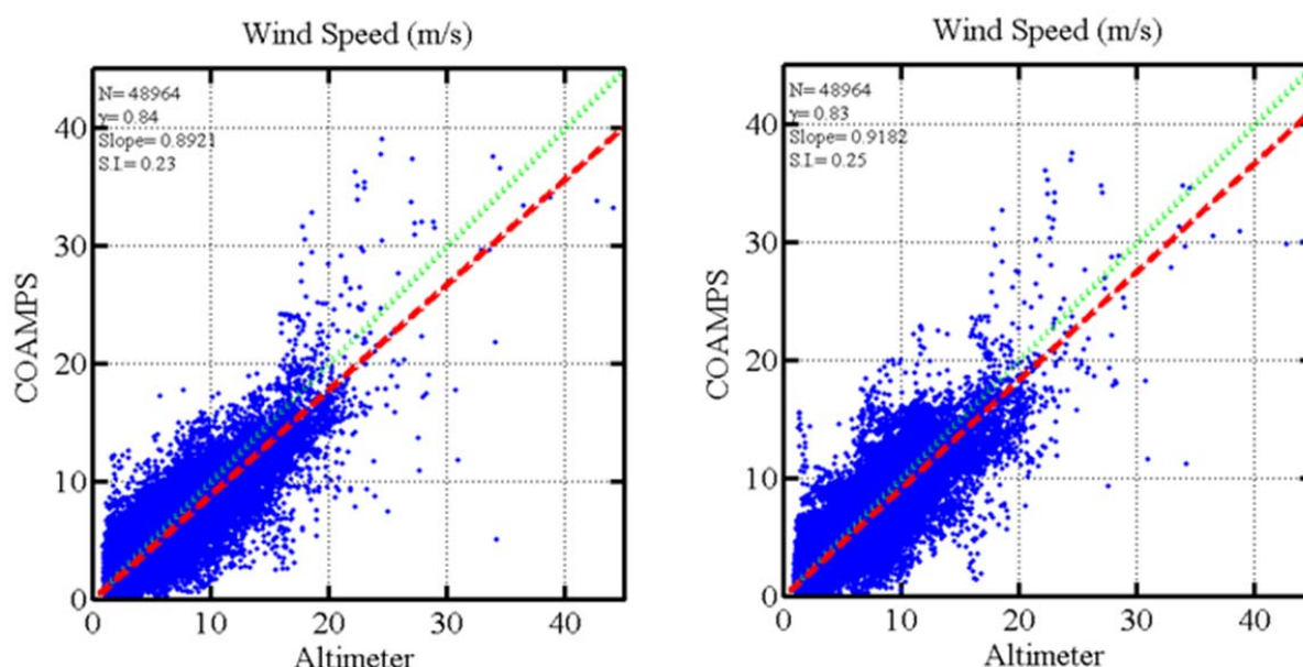
Figure 3.2-3: Comparison of uncoupled (left) and 4-way coupled (right) COAMPS wind speeds vs. altimeter data.
