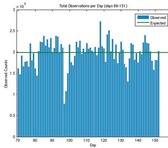
Figure 3.3-21: Total number of observations per day during Julian day 69-151 (March 10 – May 31, 2005). The green line shows the average number of daily observations.
