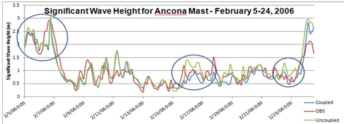
Figure 3.4-3: Bora events are captured well in the model (beginning of February). The coupled model (o2w=t, blue) showed some improvement at several distinct times during the simulation.
