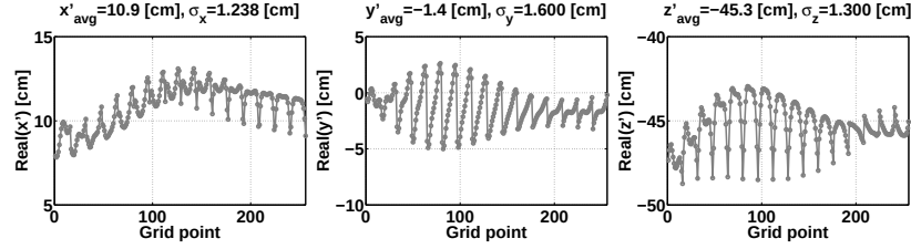
(a) 16 \times 16 points over [-50,50] \text{ cm} \times [-50,50] \text{ cm} : The results are relatively similar to the reference Fig. 1. \bar{\rho}_H = (4.39, 3.83, 5.05) \times 10^{-4} , \bar{\rho}_A = (1.7, 2.7, 3.3) \times 10^{-2} , \rho_V = 4 \times 10^{-3} .
