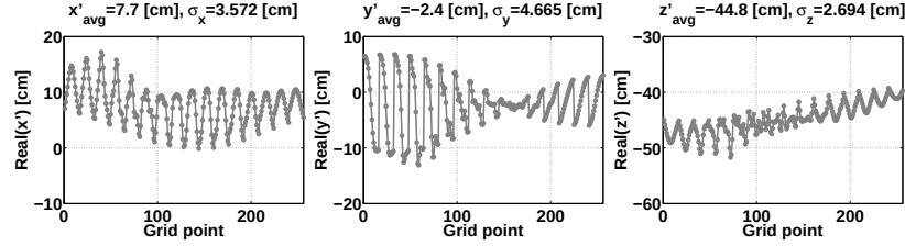
(b) 16 \times 16 points over [-100,100] \text{ cm} \times [-100,100] \text{ cm} : Increasing the size of the measurement grid does not necessarily improve the results. Most likely the fictitious grid has to be adjusted as well. \bar{\rho}_H = (0.9, 0.8, 1.4) \times 10^{-3} , \bar{\rho}_A = (0.9, 1.2, 1.6) \times 10^{-2} , \rho_V = 1 \times 10^{-3} .
