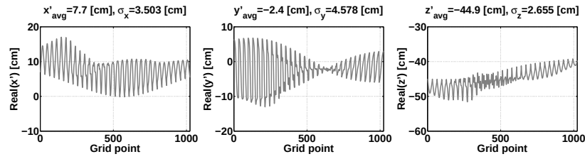
(c) 32 \times 32 points over [-100,100] \text{ cm} \times [-100,100] \text{ cm} : Same conclusion as the previous case (note that a difference inversion scheme has been used, because of computation time). \bar{\rho}_H = (1.0, 0.8, 1.3) \times 10^{-3} , \bar{\rho}_A = (0.9, 1.3, 1.6) \times 10^{-2} , \rho_V = 1 \times 10^{-3} .
