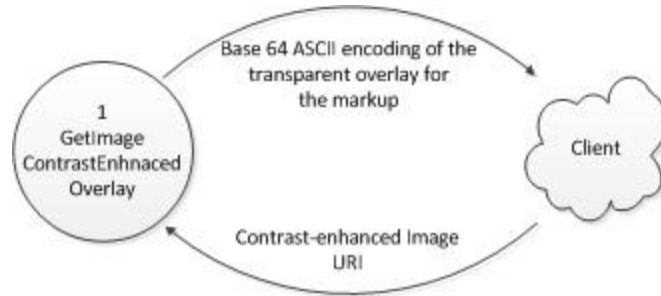
Figure 23. GetImageContrastEnhancedOverlay.
