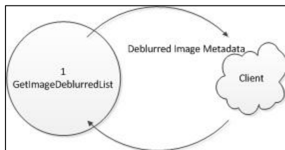
Figure 17. GetImageDeblurredList.
