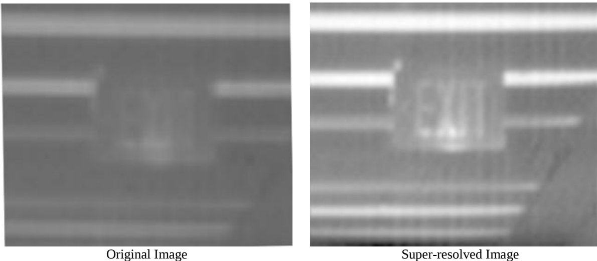
Image 4. Super-resolution.
