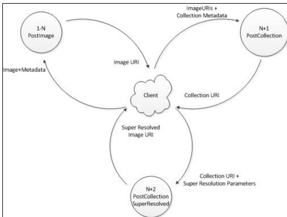
Figure 27. PostCollectionSuperResolution.
