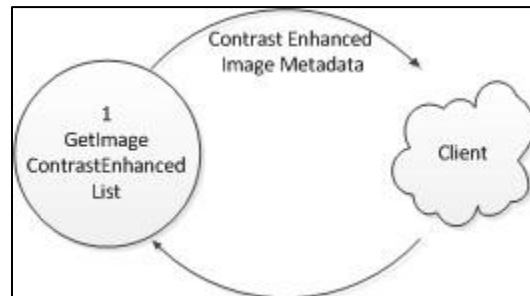
Figure 24. GetImageContrastEnhancedList.
