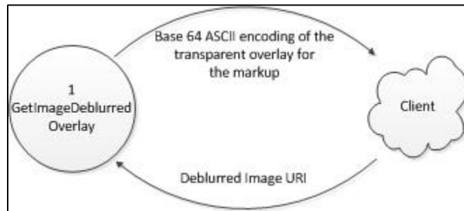
Figure 16. GetImageDeblurredOverlay.
