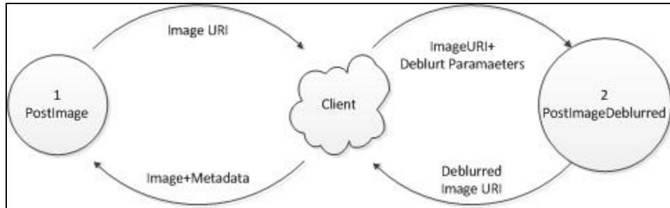
Figure 13. PostImageDeblurred.
