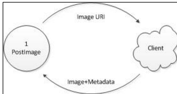
Figure 1. PostImage.
