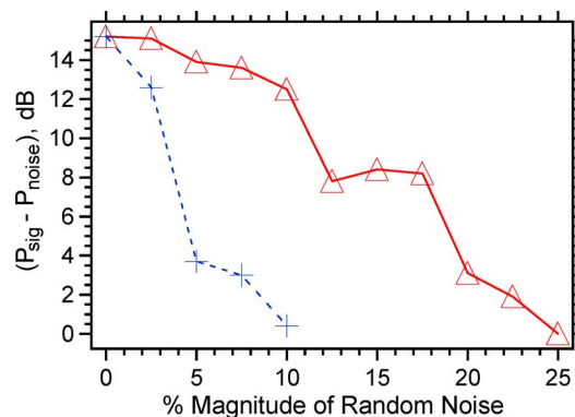
Fig. 6. Relationship between the power difference between the peak of the electrical power spectra and next strongest oscillatory peak. Blue dotted line: random noise applied to the pumping term. Red solid line: random noise applied to the injection strength term.
