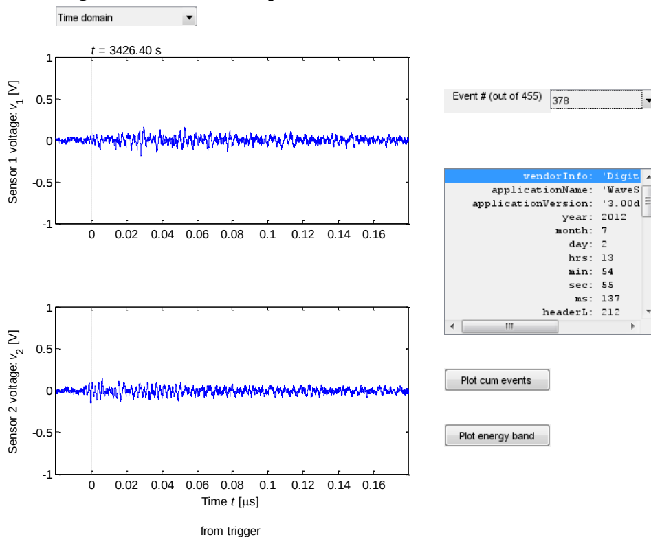
Fig. 10: MATLAB parser for AE data captured by Digital Waveform.
