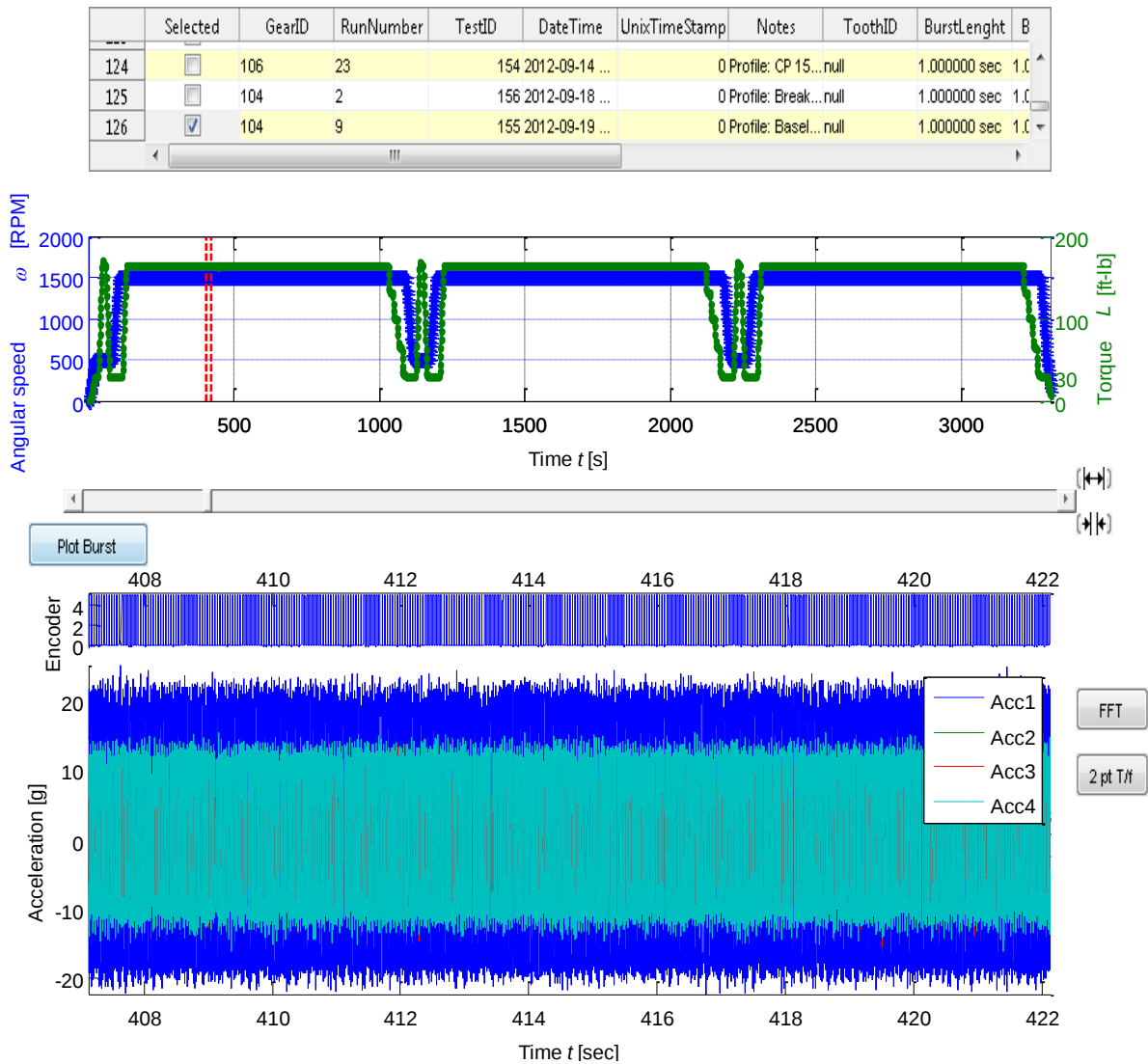
Fig. 14. Data viewer for dynamometer crack propagation. A zoomed view into the high speed data is shown in Fig. 15.
