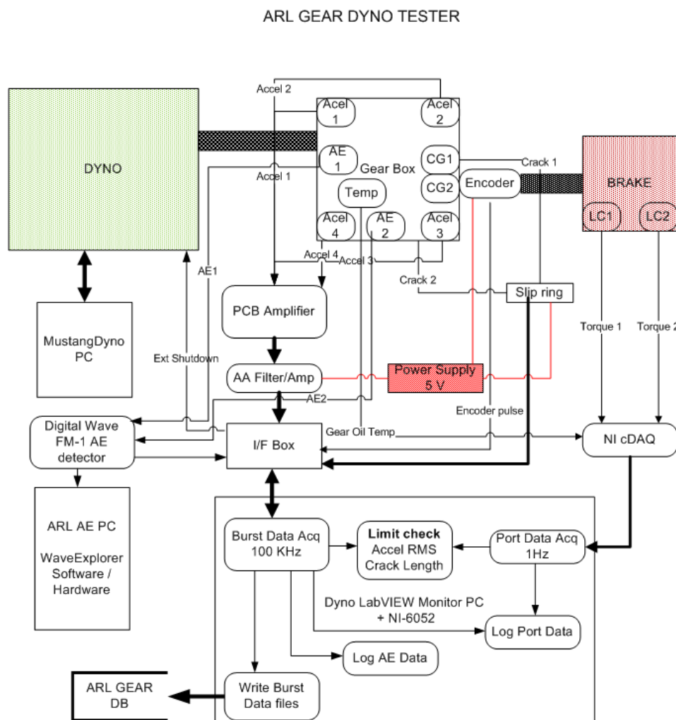
Fig. 7. Block diagram of the instrumentation system associated with the dynamometer fixture.
