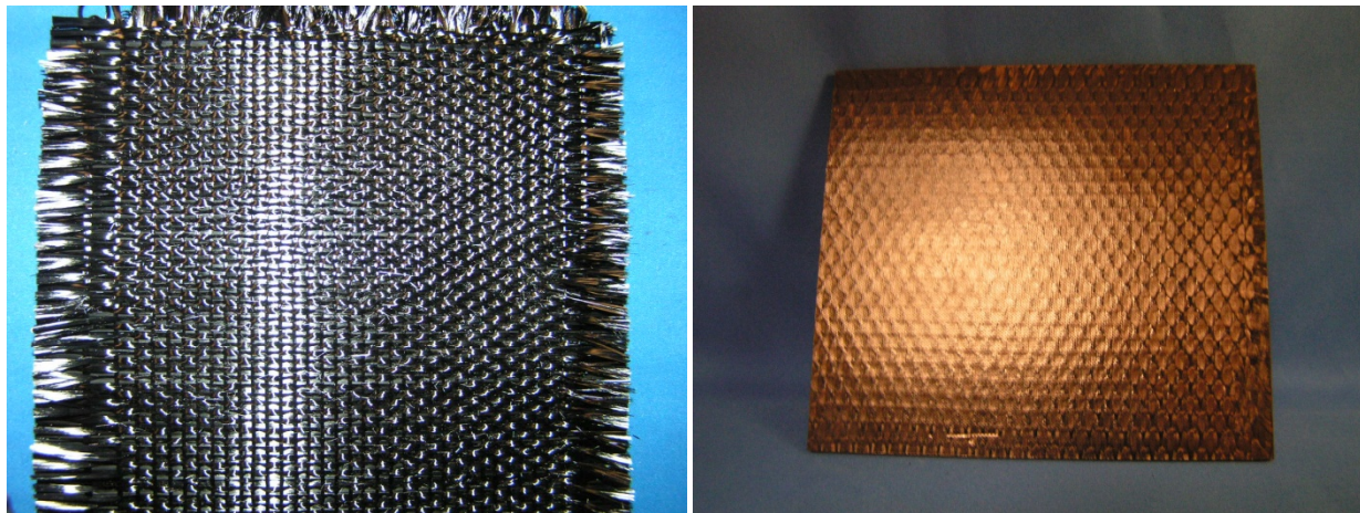
Figure 17. Three-Dimensional Pitch Fiber Preform and Fabricated Three-Dimensional Composite, Respectively
