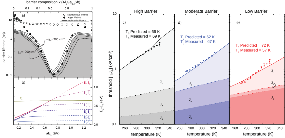
Figure 3. a) Contributions to room temperature carrier lifetime as a function of \Delta E_c . Spontaneous and Auger lifetimes are given for g_{th} = 600 \text{ cm}^{-1} . Total carrier lifetimes (including an SRH lifetime of 4.5 ns) are given for g_{th} of 200-1000 \text{cm}^{-1} . The total carrier lifetime associated with the spontaneous and Auger lifetimes plotted is emphasized with a shade underneath. b) Transition energies between the lowest conduction band state and excited states. The drop of Auger lifetime in the region that \Delta E_c \simeq E_g indicates the increased availability of states available for Auger transitions. Threshold (in equivalent current) and T_0 and contributions from the three carrier loss contributors J_{a,b,c} for c) the high barrier structure, d) the moderate barrier structure, and e) the low barrier structure.
