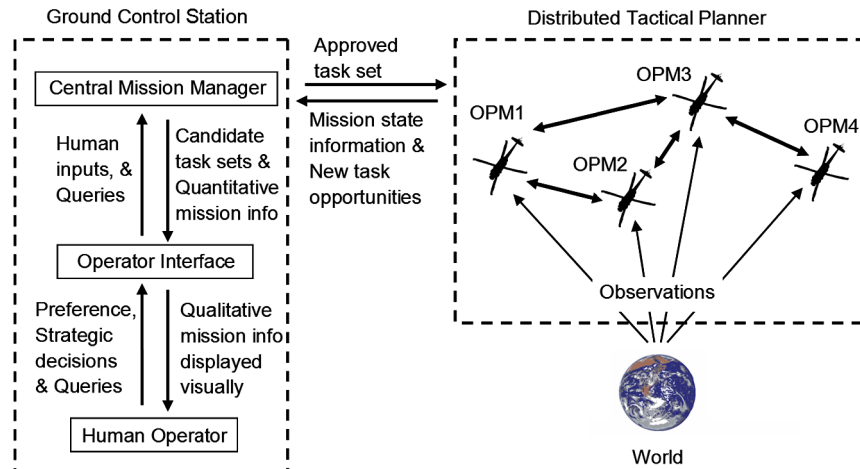
Fig. 1 OPS-USERS system architecture.
