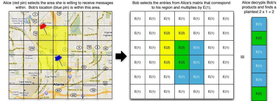
Fig. 1: Proximity Test Protocol. Alice builds a location matrix with encryptions of '1' in every entry except those that correspond to the area she is willing to receive tweets within. In her travel area, she enters encryptions of '2'. Bob selects the entries that correspond to his travel area, multiplies each entry by an encryption of '1', and returns the product to Alice. When Alice decrypts, she knows that: if any value is a '2', Bob's tweet is relevant to her. If every value is a '1', Bob's tweet is not relevant to her location.
