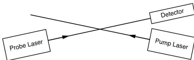
Figure 6. Schematic of pump-probe geometry for stimulated scattering measurements.
