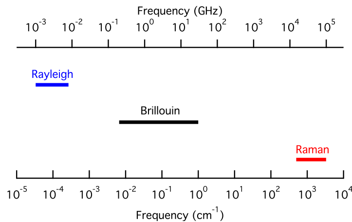
Figure 2. Frequency offset for different stimulated scattering processes.
