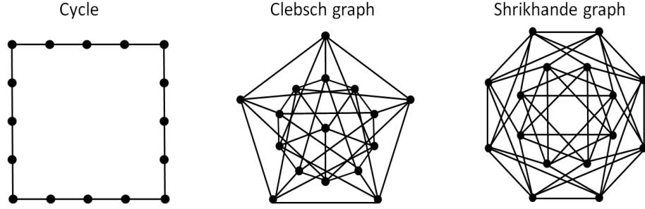
Figure 6.3. The three graphs used in the deconvolution experiments of Section 6.5.1. The Clebsch graph and the Shrikhande graph are examples of strongly regular graphs on 16 nodes [70]; see Section 6.5.1 for more details about the properties of such graphs.
