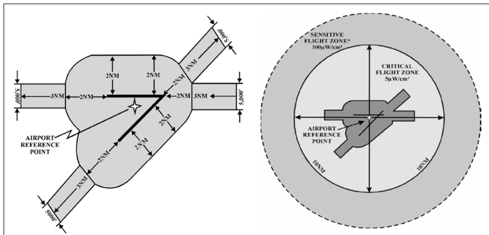
Figure 2: The LFZ (left) extends up to 2,000 feet above ground level (AGL) and 2 nautical miles (NM) in all directions from the runway centerline. It includes an additional 3-NM extension along the runway centerline. The CFZ (right) includes all airspace surrounding the LFZ within a 10-NM radius of the airport reference point, up to 10,000 feet AGL. The SFZ includes airspace outside the Laser-Free and Critical Flight Zones that authorities identify as requiring protection from the potential visual effects of laser beams. The NFZ (not depicted) include all airspace outside all other designated flight hazard zones.
