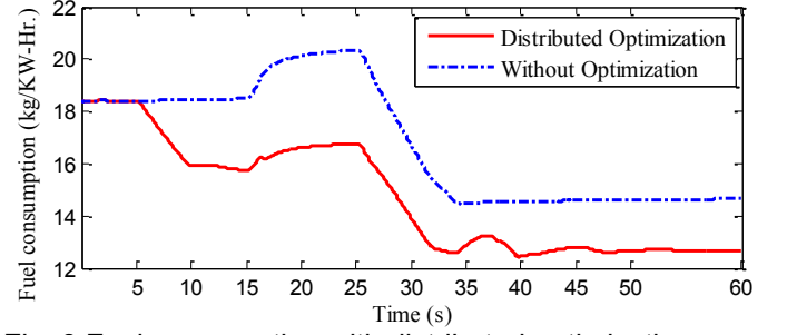
Fig. 8 Fuel consumption with distributed optimization
