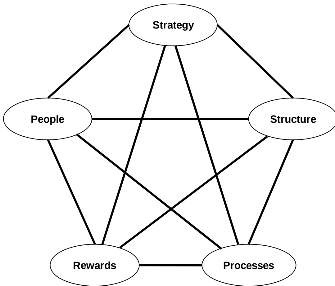
Figure C-2: Star Model [19].
