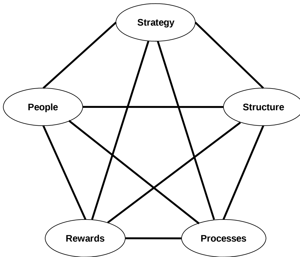
Figure 3-2: Star Model [30].
