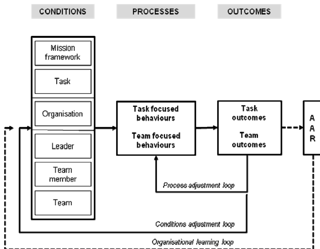
Figure 3-1: CTEF Model [28].
