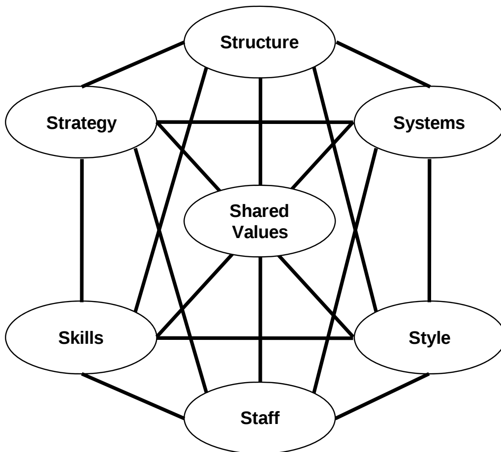
Figure 3-3: 7-S-Model [58].
