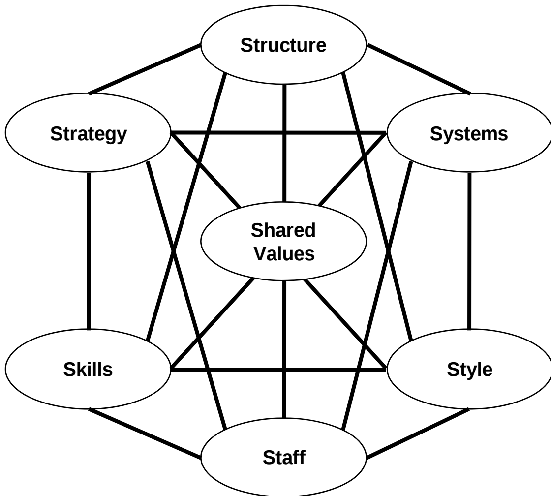
Figure C-3: 7-S-Model [37].
