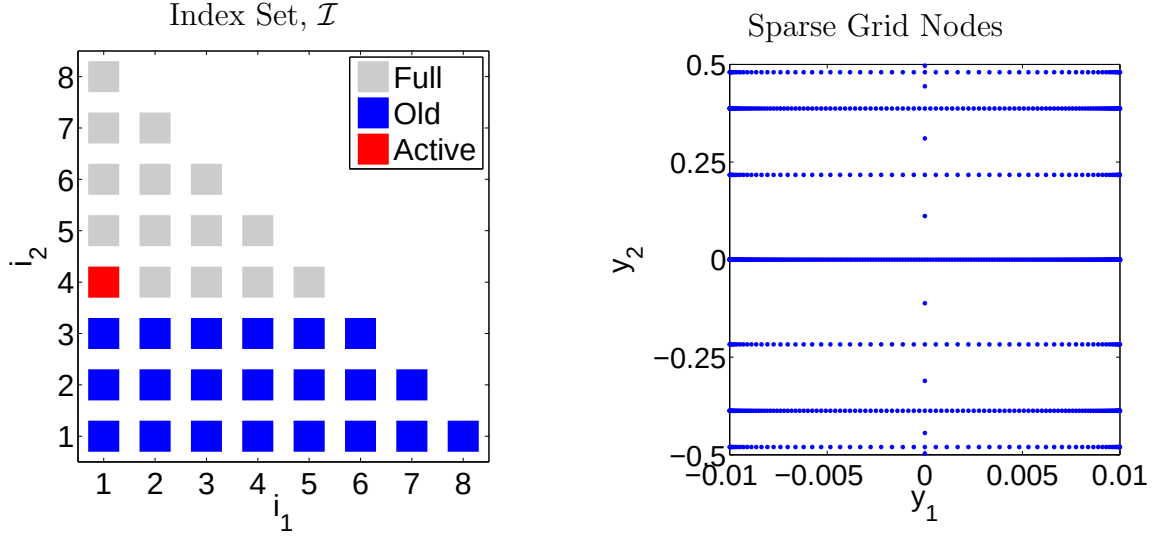
Figure 7.6: (Left) Generalized sparse grid index set. The red blocks denote “active” indices and the blue blocks denote “old” indices. The gray blocks denote the indices in the isotropic Smolyak index set of level eight. (Right) Collocation points corresponding to the index set \mathcal{I} = \mathcal{A} \cup \mathcal{O} .
