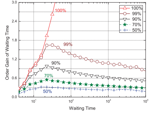
Fig. 9. Order gain of an intermittently misbehaving node in an 802.11 network with 5 legitimate nodes.
