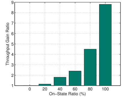
Fig. 13. Throughput ratio of the misbehaving node to a legitimate node for different on-state ratios \theta .
