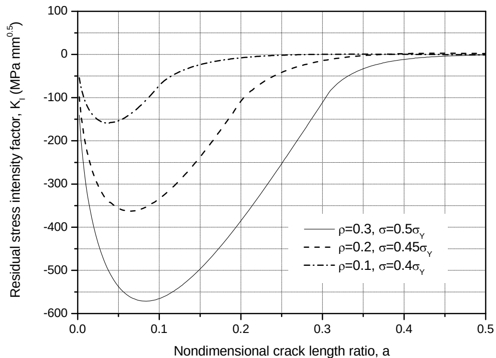
Figure 39: Stress intensity factor for a large D6ac steel plate following tension overload and unload
