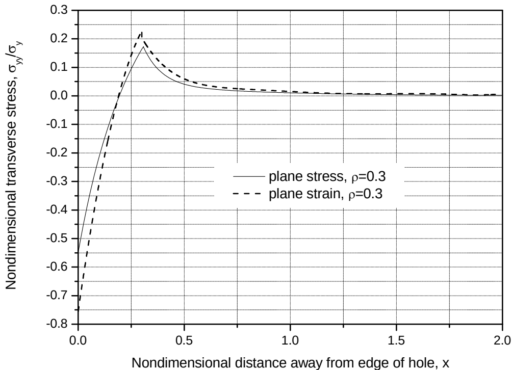
Figure 45: Comparison of transverse stresses \sigma_{yy}/\sigma_y for plane stress and plane strain for tension overload followed by unload in a large D6ac steel plate
