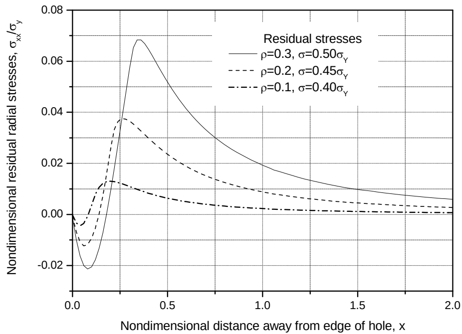
Figure 36: Residual radial stresses along prospective crack path for a large D6ac steel plate, due to remote tensile overload followed by unload
