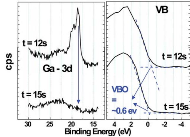
FIG. 13. VBO for sample B1 (approach B) is calculated by taking the difference in the valence band spectrum from the GaSb channel and the \text{AlAs}_y\text{Sb}_{1-y} buffer.
