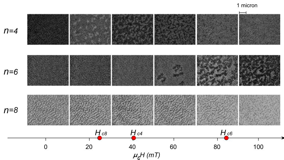
Fig. 3. Evolution of the magnetic domain structure in samples with different number of bilayer repeats as a function of the external applied magnetic field. The MTXM images were recorded at the Co L_3 edge with the field applied perpendicular to the film plane. The dots indicate the coercive fields determined from XMCD hysteresis loops (cf. Fig. 2).
