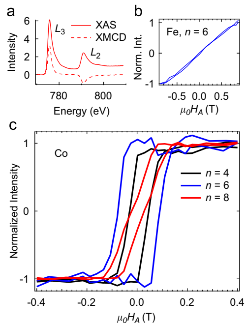
Fig. 2. (a) Energy scans of the XAS and XMCD spectra for n=8 . (b) Element specific hysteresis measurements for n=6 obtained at the Fe L_3 edge with an out-of-plane applied field, showing a hard axis magnetic response. (c) Element-specific hysteresis loops for different bilayer repeats obtained at the Co L_3 absorption edge using out-of-plane applied magnetic fields.
