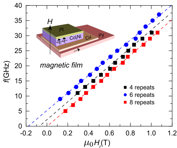
Fig. 1. FMR results: frequency dependence of the resonant field versus applied field perpendicular to the film plane. The dashed lines are fits using Eq. (1). The inset shows a schematic of the sample layer stack and the magnetic moments orientations of Co|Ni and Py layers.
