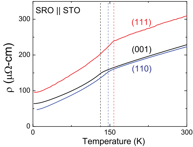
FIG. 6. (Color online) Resistivity ( \rho ) vs. temperature for 65-nm-thick films on (100), (110), and (111) STO showing significant variation in resistivity and transition temperature among the different orientations. The dashed lines mark the resistivity kink, and, thus, transition temperature, of the corresponding film.
