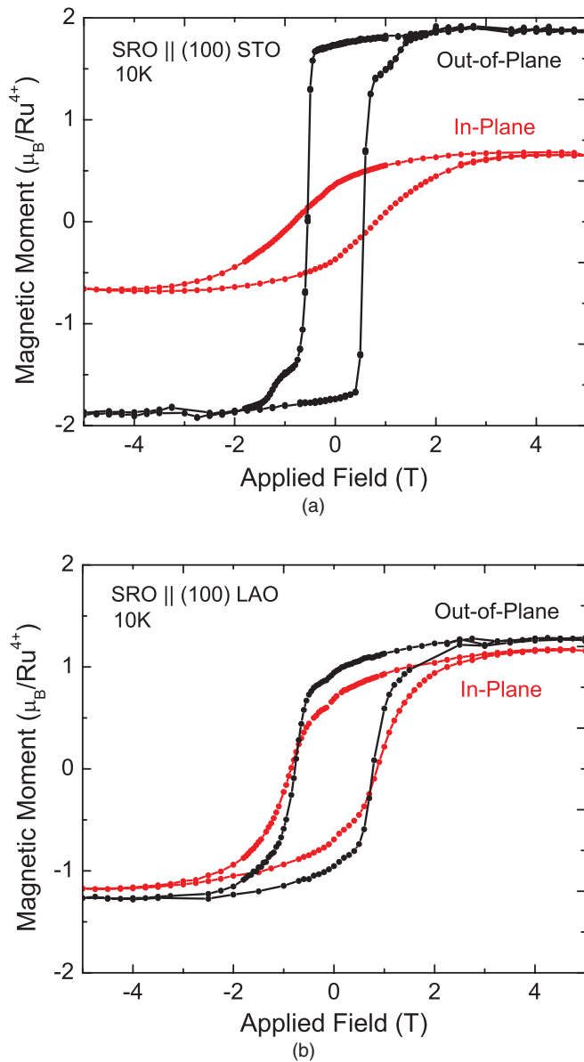
FIG. 3. (Color online) Magnetic moment vs. applied field at 10 K with external field in the in-plane and out-of-plane directions for (a) coherently strained SRO on (100) STO and (b) relaxed SRO on (100) LAO.
