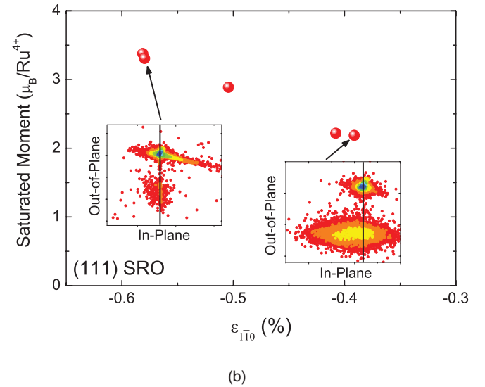
FIG. 2. (Color online) Saturated magnetic moment vs. strain for films on (a) (100)-oriented STO, LSAT, and LAO and (b) (111)-oriented STO. Thicknesses range from 20 to 120 nm. Strain values extracted from the 301 and 312 reflections, respectively, show that as compressive in-plane strain increases, (100)-oriented films approach a saturated magnetic moment of 2 \mu_B/\text{Ru}^{4+} while (111)-oriented films approach a saturated moment of 4 \mu_B/\text{Ru}^{4+} . (Insets) RLMs of several films further demonstrate that it is the lattice distortion that determines the magnetic state.
