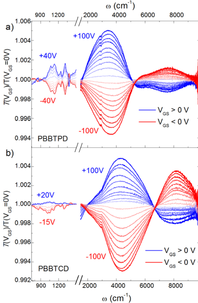
Figure 2: Voltage-induced change in transmission spectra T(\omega, V_{GS})/T(\omega, V_{GS} = 0 \text{ V}) for structures employing (a) PBBTPD and (b) PBBTCD as the active semiconductor. Blue curves indicate n-type operation ( V_{GS} > 0 \text{ V} ); red curves indicate p-type operation ( V_{GS} < 0 \text{ V} ).
