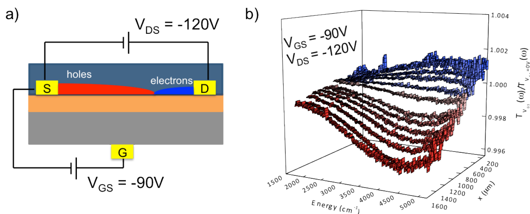
Figure 3: a) Schematic of OFET biased in “ambipolar” mode of operation. b) Voltage-induced change in transmission spectra T(\omega, V_{GS})/T(\omega, V_{GS} = 0 \text{ V}) for PBBTPD OFET across the conduction channel. Red (blue) curves indicate a negative (positive) electrical potential in the channel.
