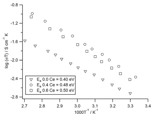
Fig. 6. Arrhenius data for the hot pressed specimens with the following compositions where: x = 0.0, 0.4 and 0.6 Ce in the formula: \text{Li}_{7-x}\text{La}_{3-x}\text{Ce}_x\text{Zr}_2\text{O}_{12} . Measurements were made between 298 K and 373 K.
