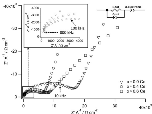
Fig. 5. Nyquist plots for the hot pressed specimens where: x = 0.0, 0.4 and 0.6 Ce in the formula: \text{Li}_{7-x}\text{La}_{3-x}\text{Ce}_x\text{Zr}_2\text{O}_{12} . The inset highlights the high frequency intercept. The equivalent circuit utilized for obtaining the conductivities is also included.
