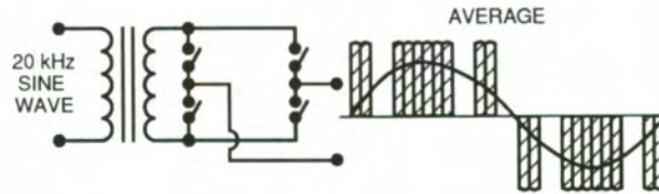
Figure 3. - Waveshape synthesis.
