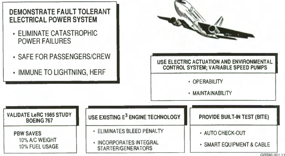
FIGURE 1. - MAJOR TASKS AND BENEFITS OF POWER-BY-WIRE TECHNOLOGY.
