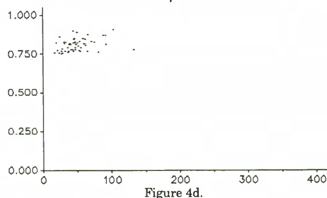
Figure 4. Target letter A. Filtered structuring elements. The horizontal and vertical axes record complexity and performance, respectively. Better performers are filtered from the total population using the "good" criteria, i.e. \alpha > .75 and \beta > .75 . The top pair are filtered by requiring "good" performance with the training set. The bottom pair are filtered by requiring "good" performance with both the training and test sets.
